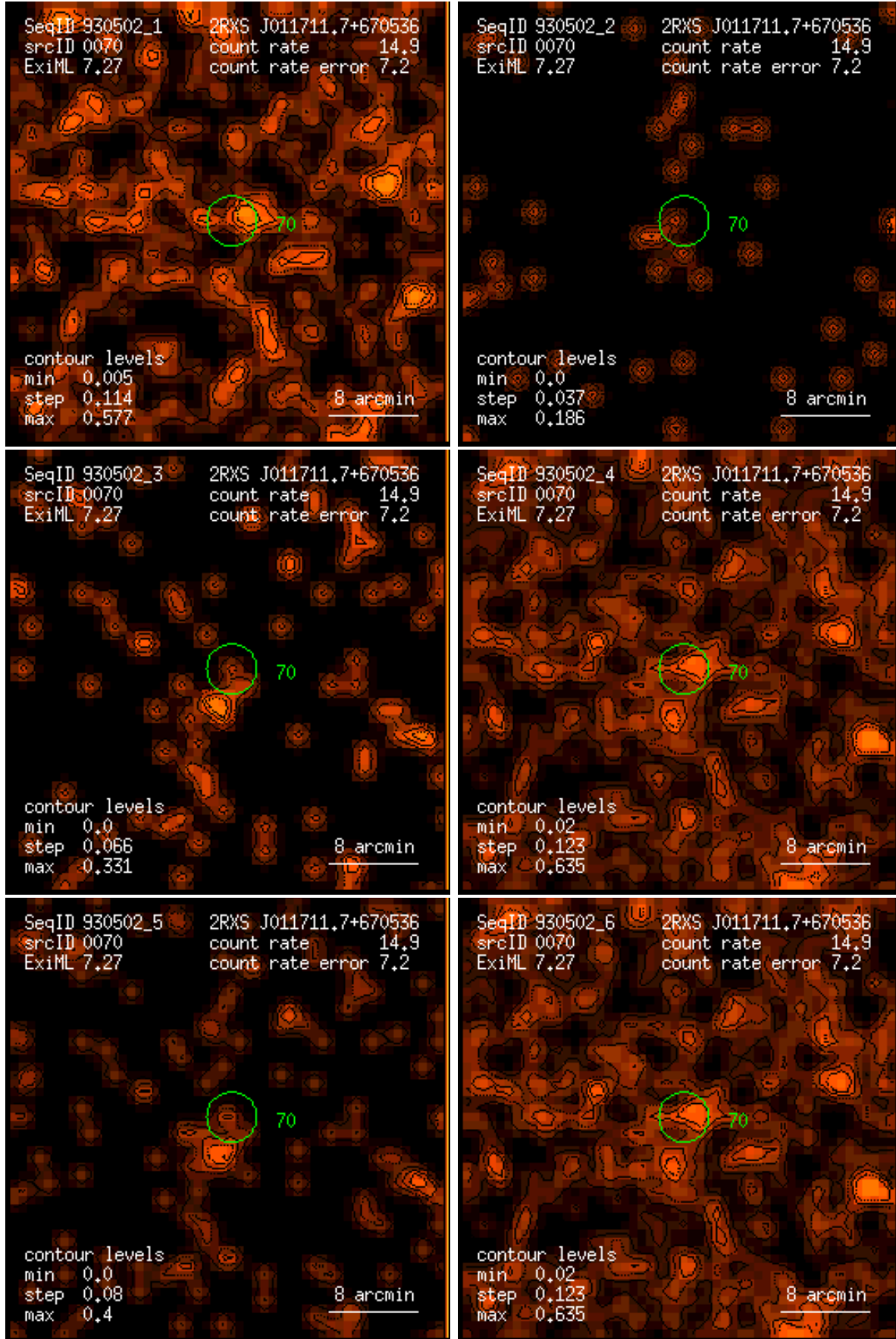
Figure 70: RASS 930502: detection 0070: band rate images, Gaussian filter: (1) PSPC channels 11 – 41, (2) 52 – 90, (3) 91 – 201, (4) 11 – 235, (5) 52 – 201, (6) 11 – 201. Broad band rates in counts/ks. Band rate contour levels in counts/ks/arcmin 2 .
