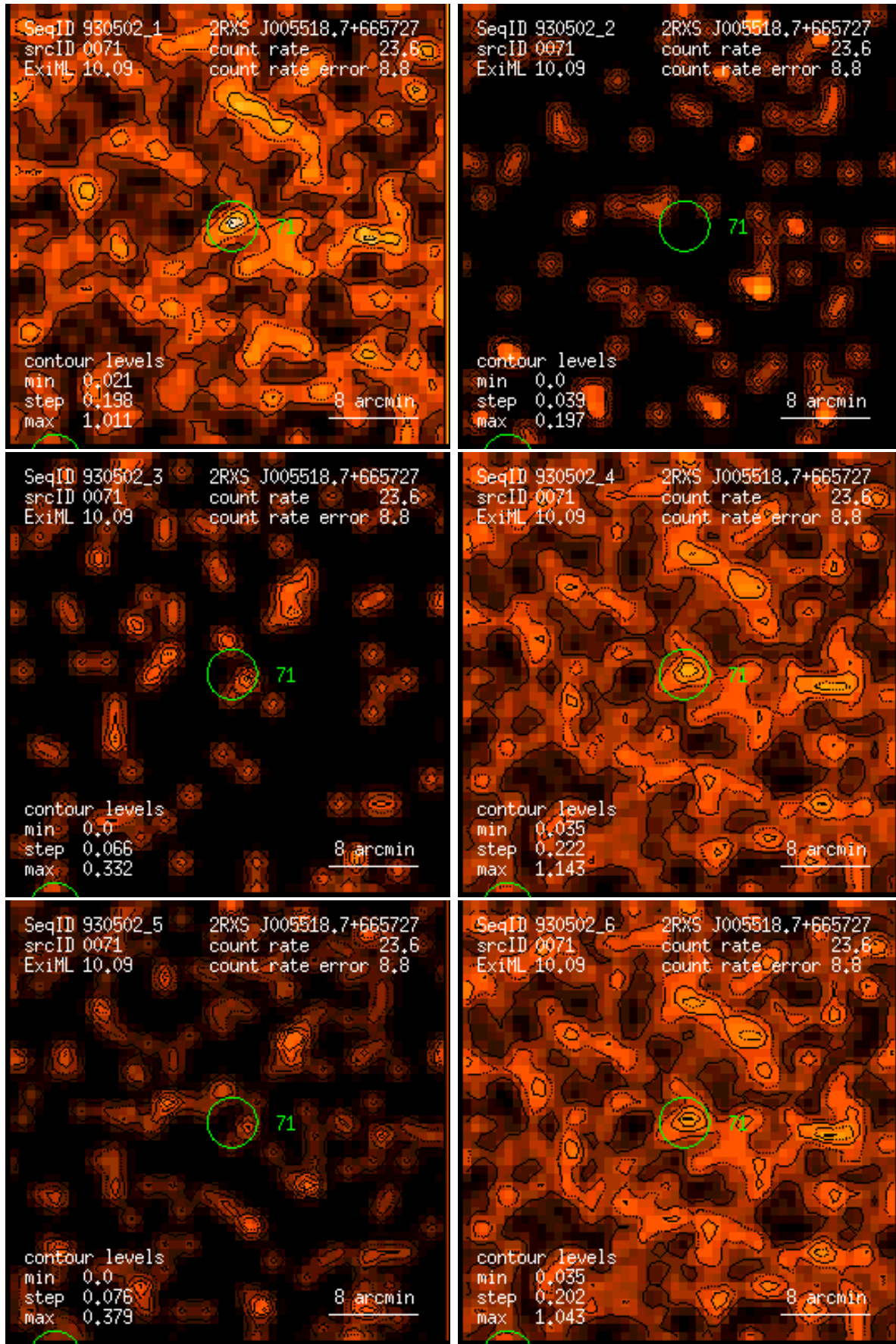
Figure 71: RASS 930502: detection 0071: band rate images, Gaussian filter: (1) PSPC channels 11 – 41, (2) 52 – 90, (3) 91 – 201, (4) 11 – 235, (5) 52 – 201, (6) 11 – 201. Broad band rates in counts/ks. Band rate contour levels in counts/ks/arcmin 2 .
