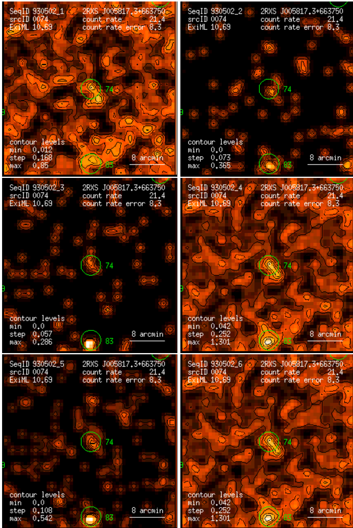
Figure 74: RASS 930502: detection 0074: band rate images, Gaussian filter: (1) PSPC channels 11 – 41, (2) 52 – 90, (3) 91 – 201, (4) 11 – 235, (5) 52 – 201, (6) 11 – 201. Broad band rates in counts/ks. Band rate contour levels in counts/ks/arcmin 2 .
