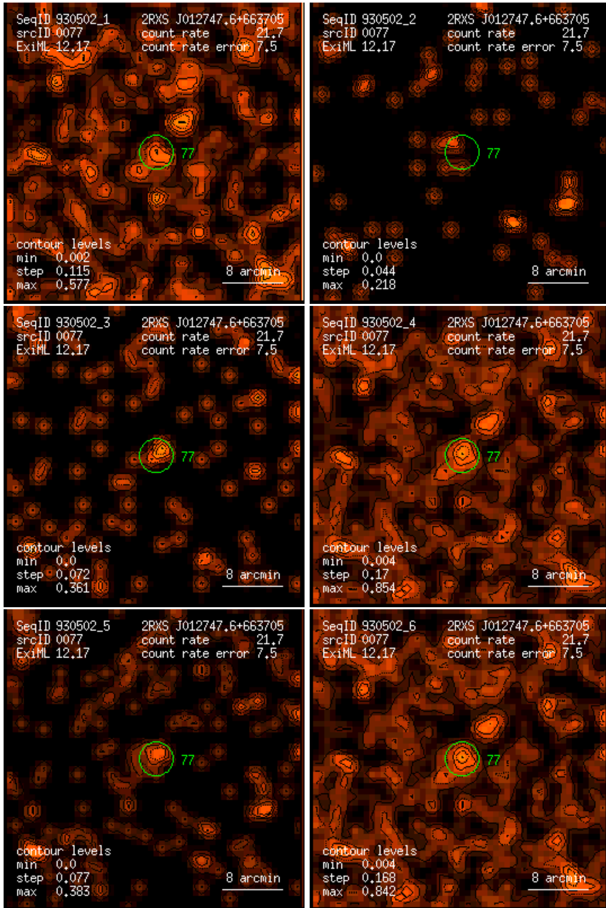
Figure 77: RASS 930502: detection 0077: band rate images, Gaussian filter: (1) PSPC channels 11 – 41, (2) 52 – 90, (3) 91 – 201, (4) 11 – 235, (5) 52 – 201, (6) 11 – 201. Broad band rates in counts/ks. Band rate contour levels in counts/ks/arcmin 2 .
