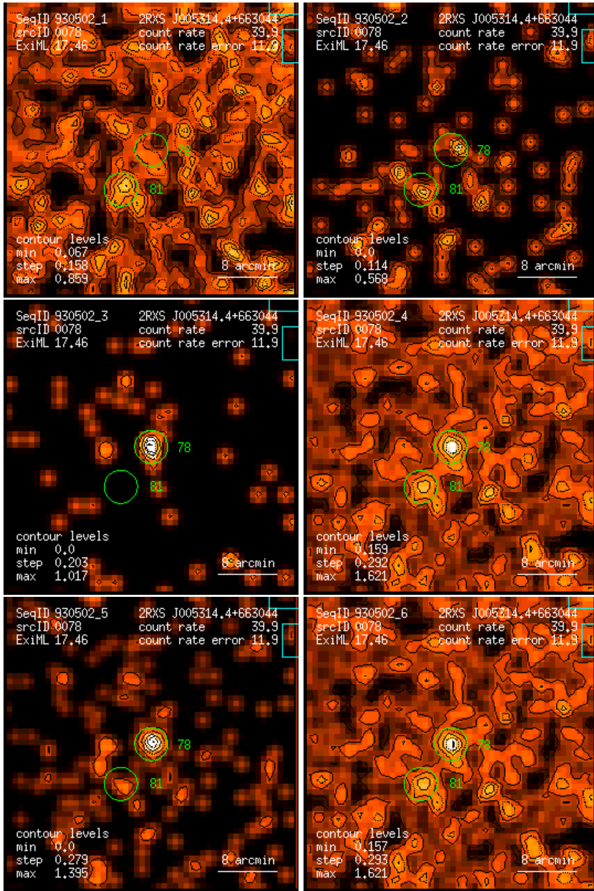
Figure 78: RASS 930502: detection 0078: band rate images, Gaussian filter: (1) PSPC channels 11 – 41, (2) 52 – 90, (3) 91 – 201, (4) 11 – 235, (5) 52 – 201, (6) 11 – 201. Broad band rates in counts/ks. Band rate contour levels in counts/ks/arcmin 2 .
