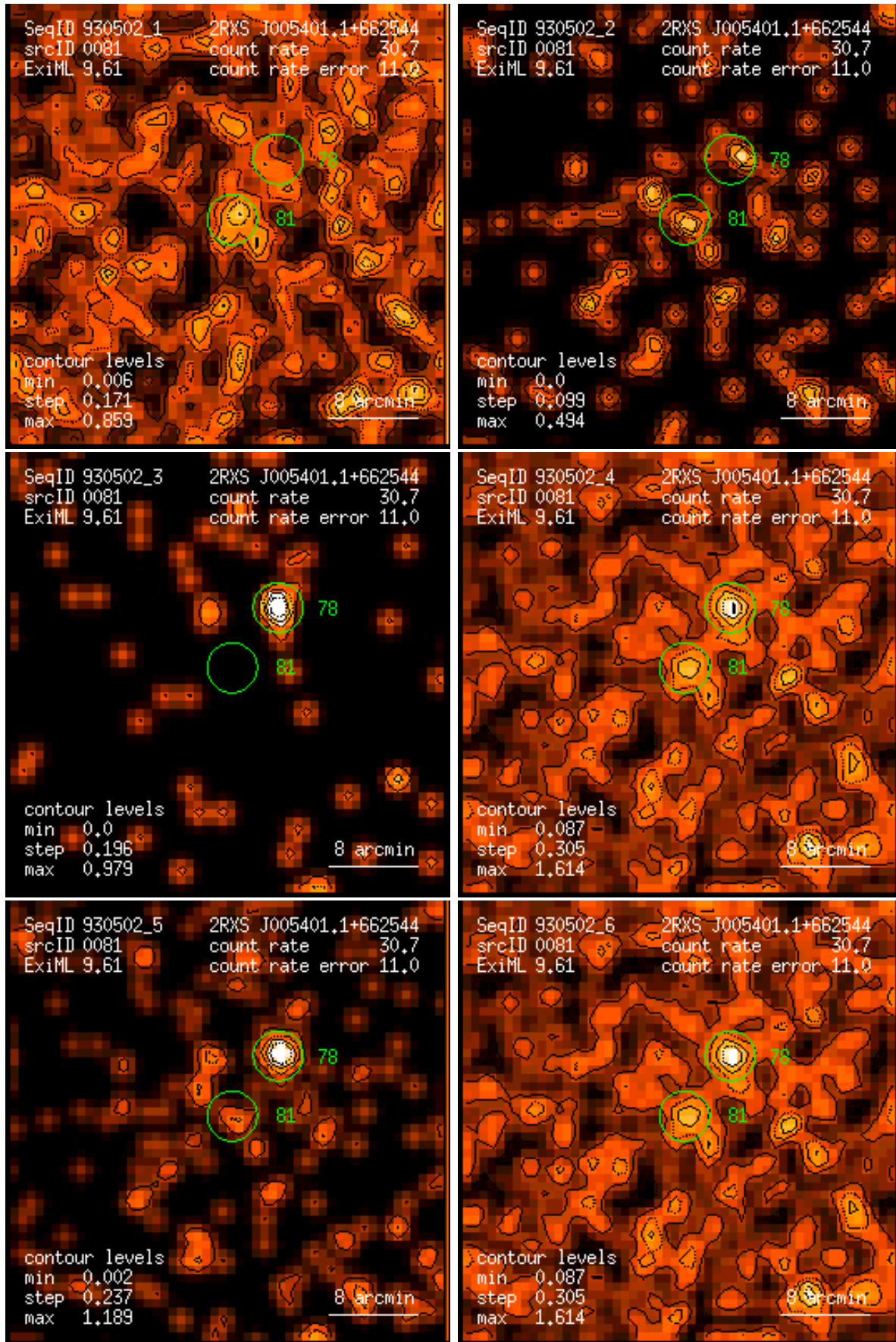
Figure 81: RASS 930502: detection 0081: band rate images, Gaussian filter: (1) PSPC channels 11 – 41, (2) 52 – 90, (3) 91 – 201, (4) 11 – 235, (5) 52 – 201, (6) 11 – 201. Broad band rates in counts/ks. Band rate contour levels in counts/ks/arcmin 2 .
