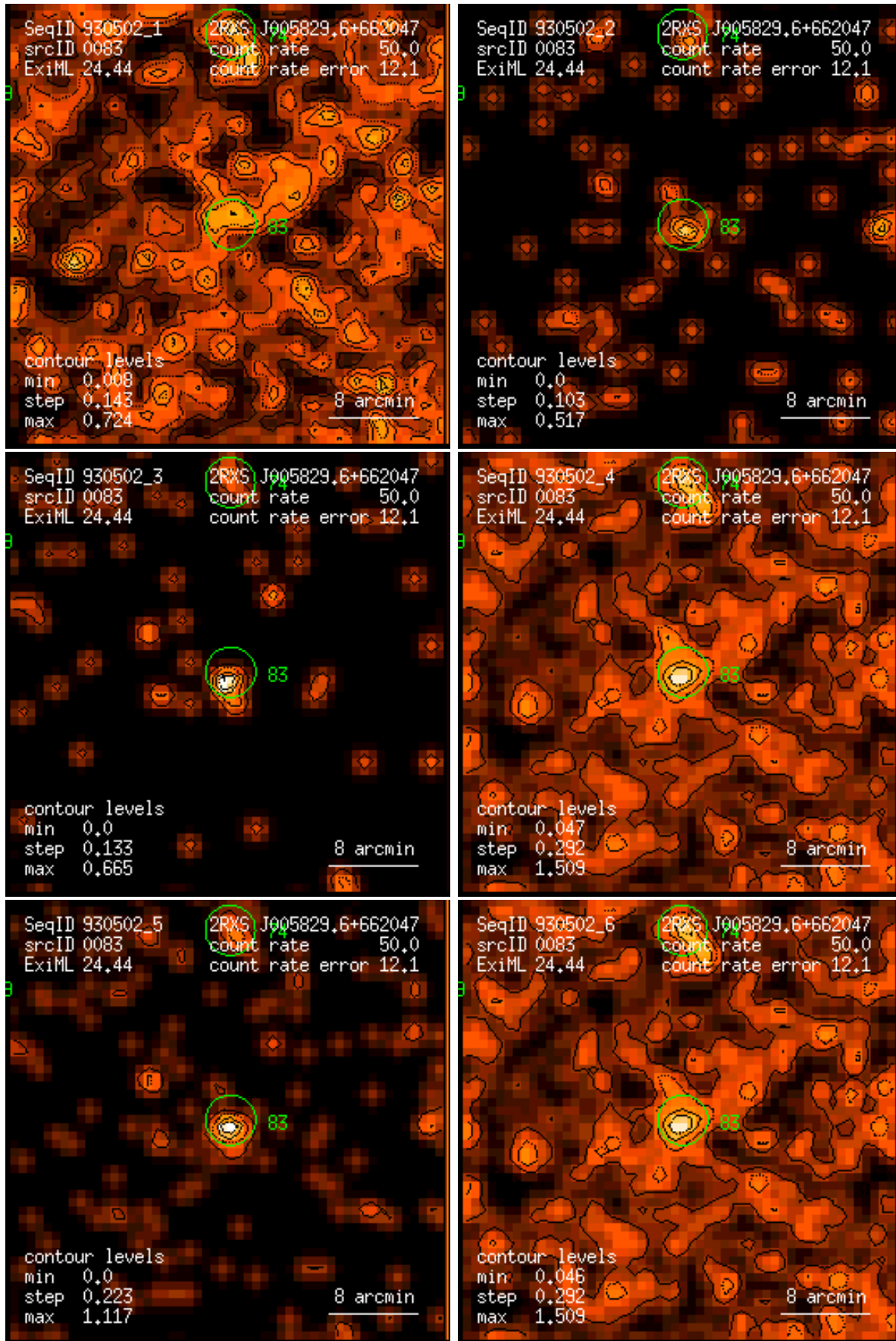
Figure 83: RASS 930502: detection 0083: band rate images, Gaussian filter: (1) PSPC channels 11 – 41, (2) 52 – 90, (3) 91 – 201, (4) 11 – 235, (5) 52 – 201, (6) 11 – 201. Broad band rates in counts/ks. Band rate contour levels in counts/ks/arcmin 2 .
