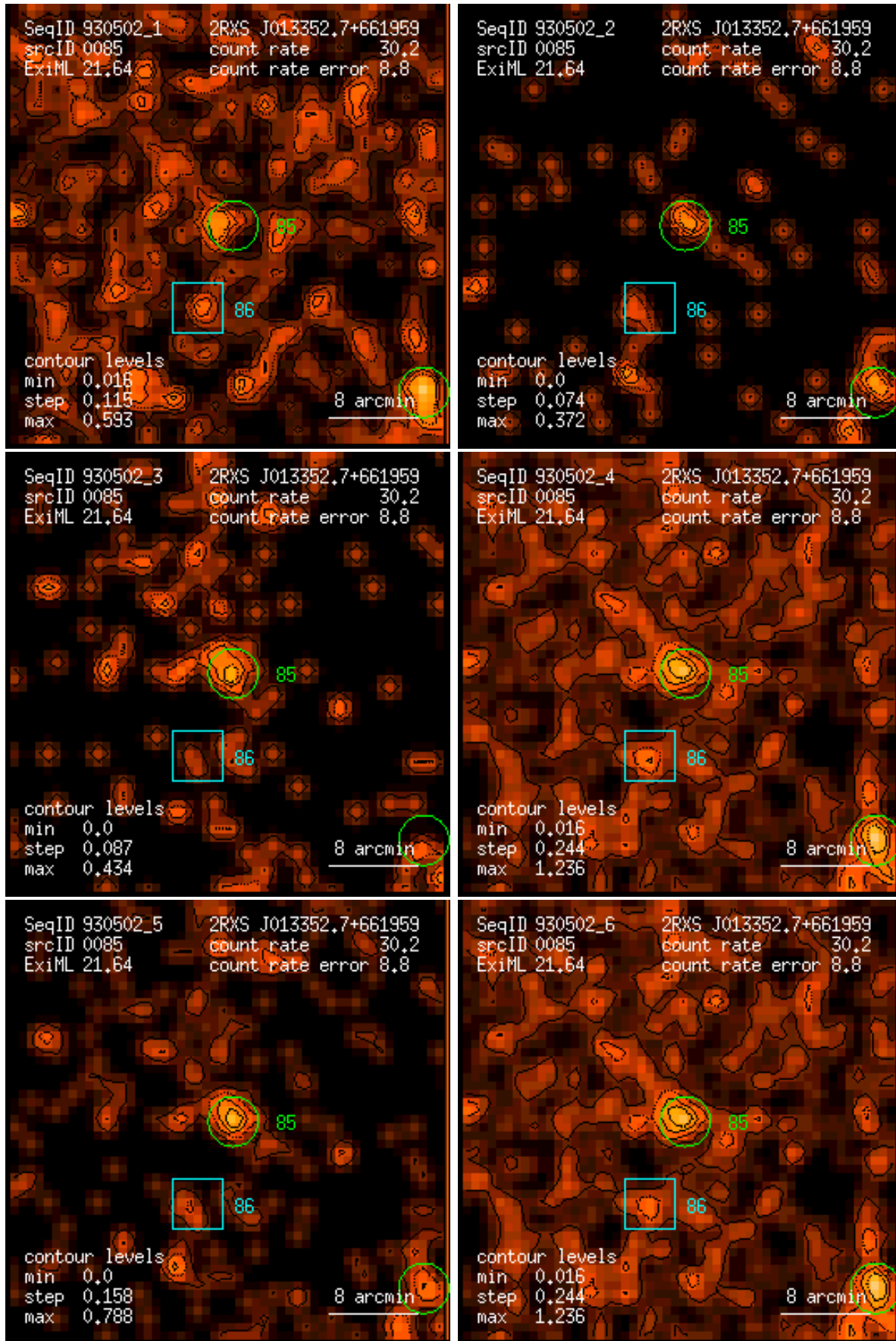
Figure 85: RASS 930502: detection 0085: band rate images, Gaussian filter: (1) PSPC channels 11 – 41, (2) 52 – 90, (3) 91 – 201, (4) 11 – 235, (5) 52 – 201, (6) 11 – 201. Broad band rates in counts/ks. Band rate contour levels in counts/ks/arcmin 2 .
