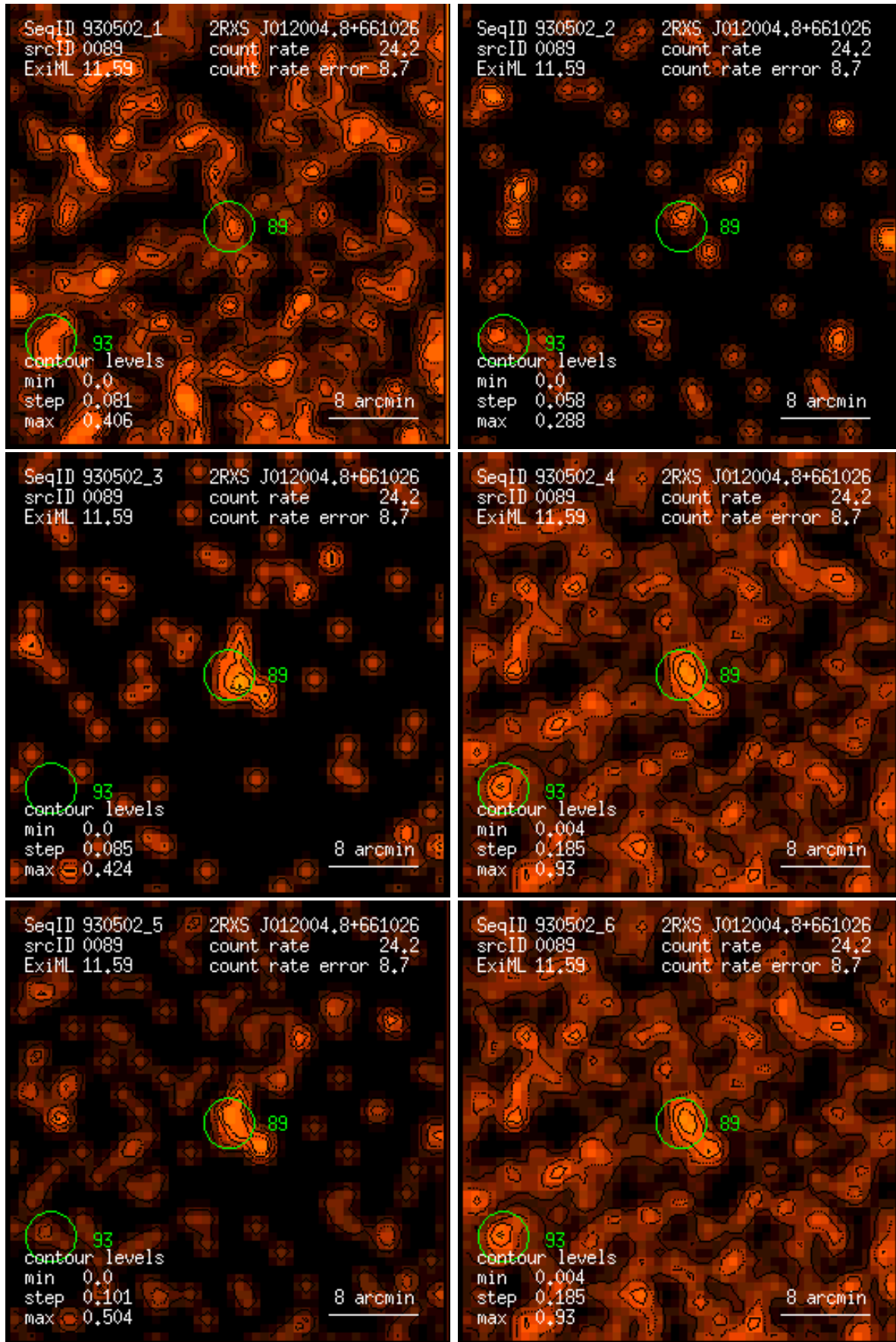
Figure 89: RASS 930502: detection 0089: band rate images, Gaussian filter: (1) PSPC channels 11 – 41, (2) 52 – 90, (3) 91 – 201, (4) 11 – 235, (5) 52 – 201, (6) 11 – 201. Broad band rates in counts/ks. Band rate contour levels in counts/ks/arcmin 2 .
