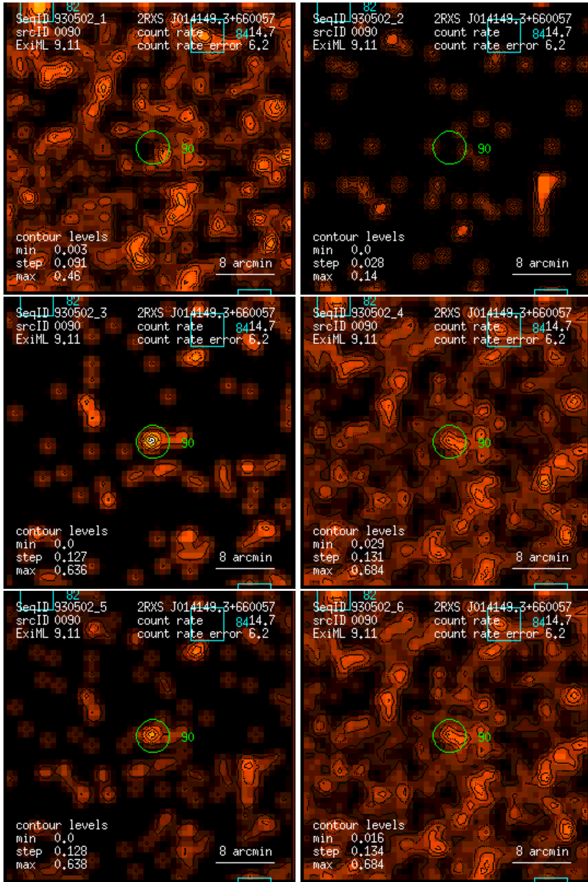
Figure 90: RASS 930502: detection 0090: band rate images, Gaussian filter: (1) PSPC channels 11 – 41, (2) 52 – 90, (3) 91 – 201, (4) 11 – 235, (5) 52 – 201, (6) 11 – 201. Broad band rates in counts/ks. Band rate contour levels in counts/ks/arcmin 2 .
