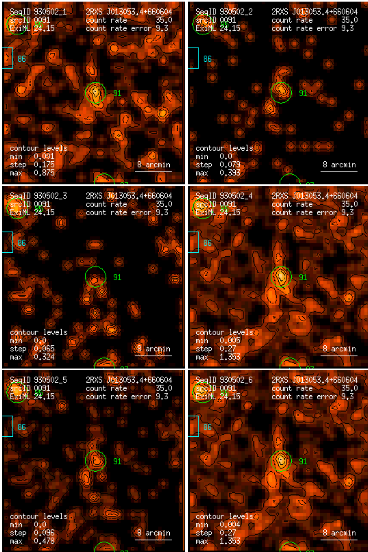
Figure 91: RASS 930502: detection 0091: band rate images, Gaussian filter: (1) PSPC channels 11 – 41, (2) 52 – 90, (3) 91 – 201, (4) 11 – 235, (5) 52 – 201, (6) 11 – 201. Broad band rates in counts/ks. Band rate contour levels in counts/ks/arcmin 2 .
