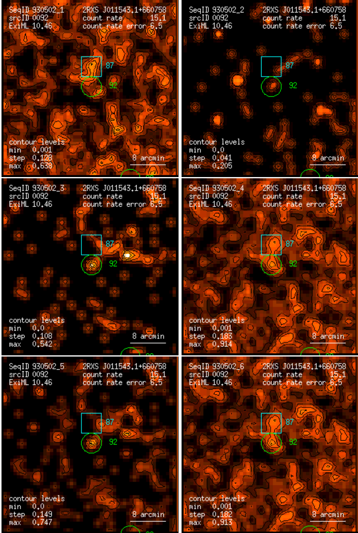
Figure 92: RASS 930502: detection 0092: band rate images, Gaussian filter: (1) PSPC channels 11 – 41, (2) 52 – 90, (3) 91 – 201, (4) 11 – 235, (5) 52 – 201, (6) 11 – 201. Broad band rates in counts/ks. Band rate contour levels in counts/ks/arcmin 2 .
