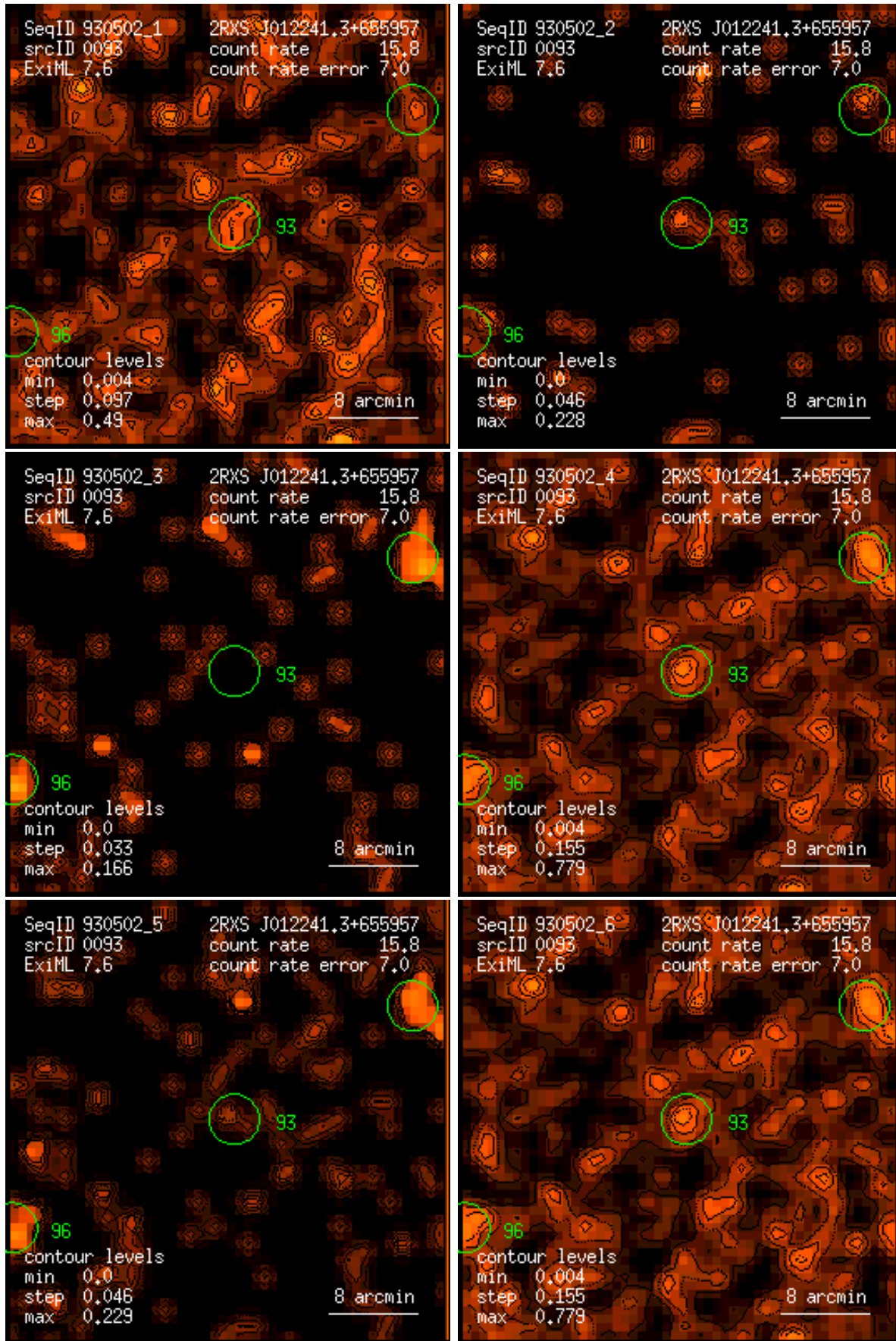
Figure 93: RASS 930502: detection 0093: band rate images, Gaussian filter: (1) PSPC channels 11 – 41, (2) 52 – 90, (3) 91 – 201, (4) 11 – 235, (5) 52 – 201, (6) 11 – 201. Broad band rates in counts/ks. Band rate contour levels in counts/ks/arcmin 2 .
