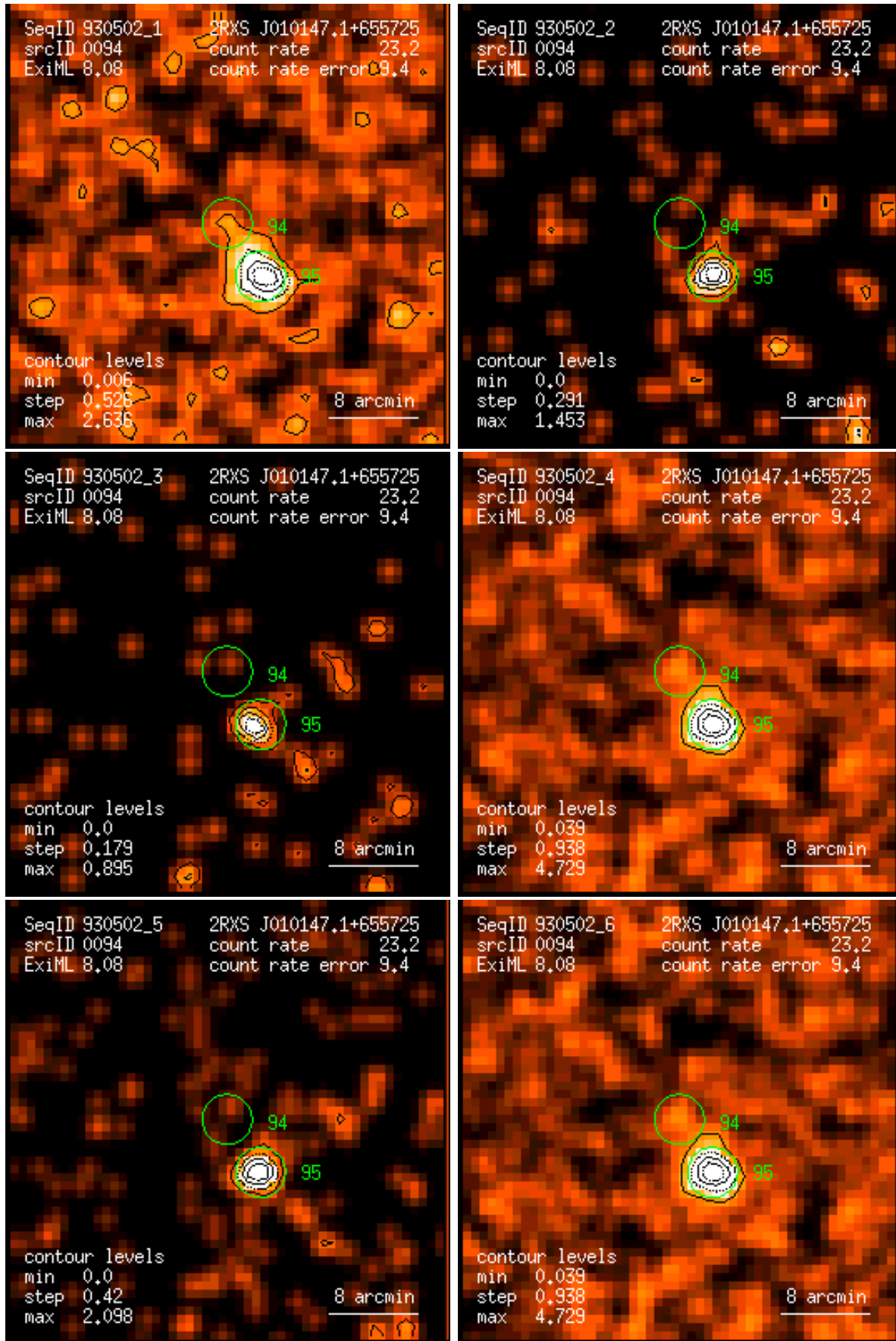
Figure 94: RASS 930502: detection 0094: band rate images, Gaussian filter: (1) PSPC channels 11 – 41, (2) 52 – 90, (3) 91 – 201, (4) 11 – 235, (5) 52 – 201, (6) 11 – 201. Broad band rates in counts/ks. Band rate contour levels in counts/ks/arcmin 2 .
