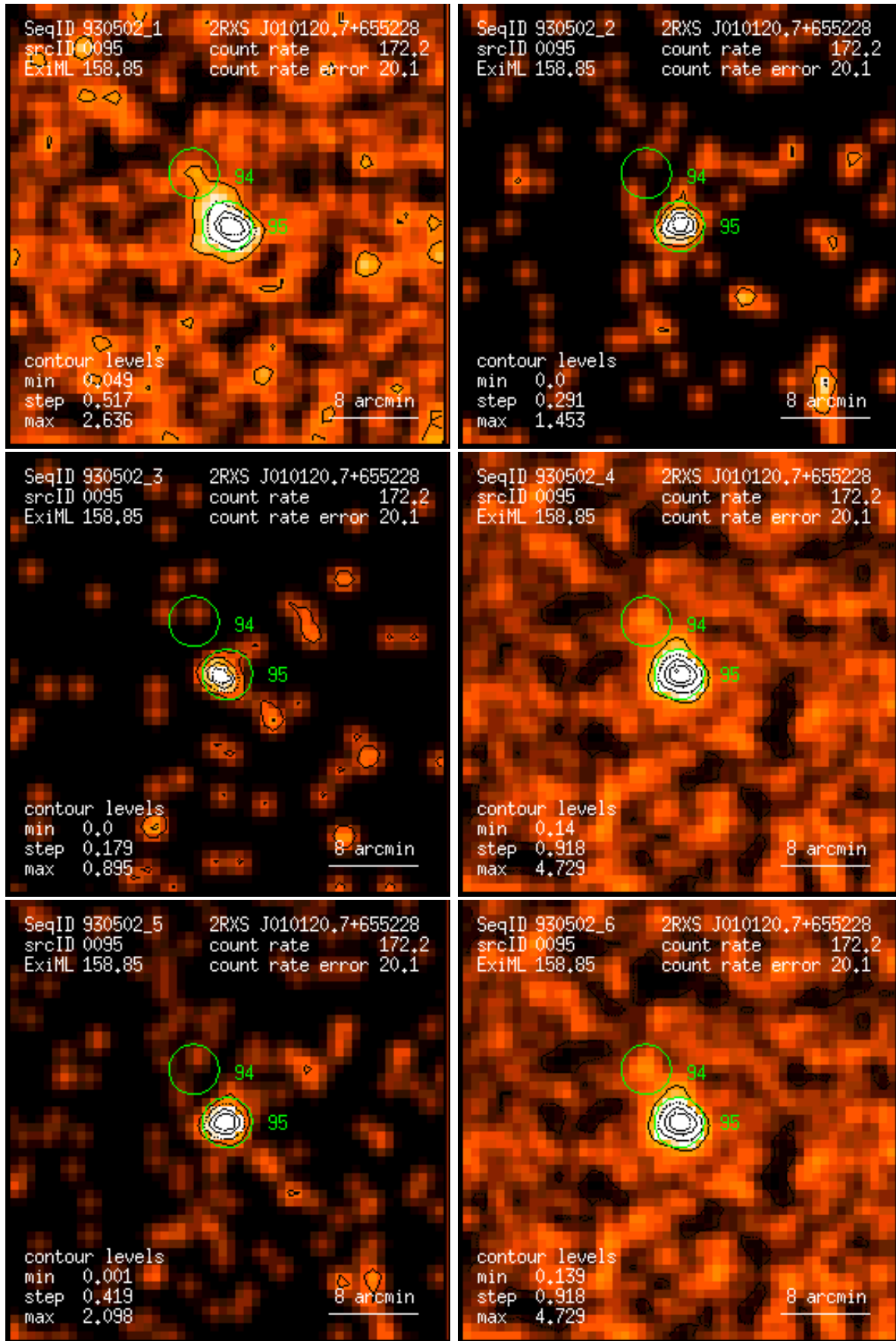
Figure 95: RASS 930502: detection 0095: band rate images, Gaussian filter: (1) PSPC channels 11 – 41, (2) 52 – 90, (3) 91 – 201, (4) 11 – 235, (5) 52 – 201, (6) 11 – 201. Broad band rates in counts/ks. Band rate contour levels in counts/ks/arcmin 2 .
