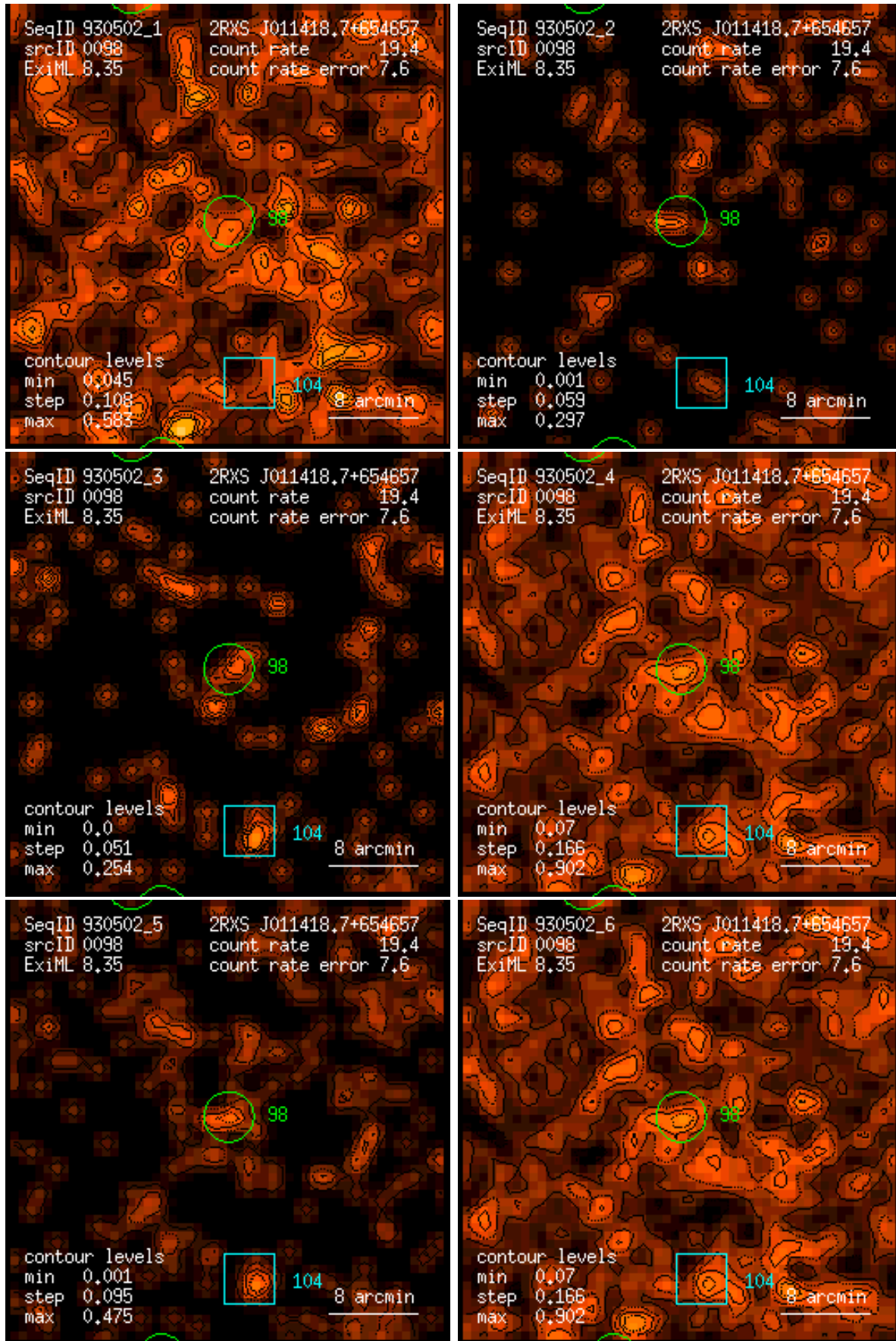
Figure 98: RASS 930502: detection 0098: band rate images, Gaussian filter: (1) PSPC channels 11 – 41, (2) 52 – 90, (3) 91 – 201, (4) 11 – 235, (5) 52 – 201, (6) 11 – 201. Broad band rates in counts/ks. Band rate contour levels in counts/ks/arcmin 2 .
