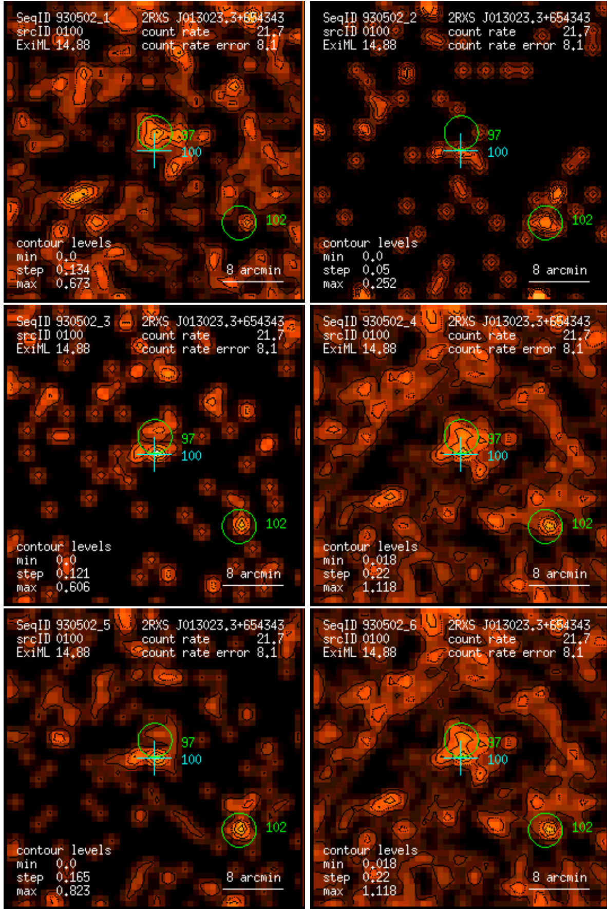
Figure 100: RASS 930502: detection 0100: band rate images, Gaussian filter: (1) PSPC channels 11 – 41, (2) 52 – 90, (3) 91 – 201, (4) 11 – 235, (5) 52 – 201, (6) 11 – 201. Broad band rates in counts/ks. Band rate contour levels in counts/ks/arcmin 2 .
