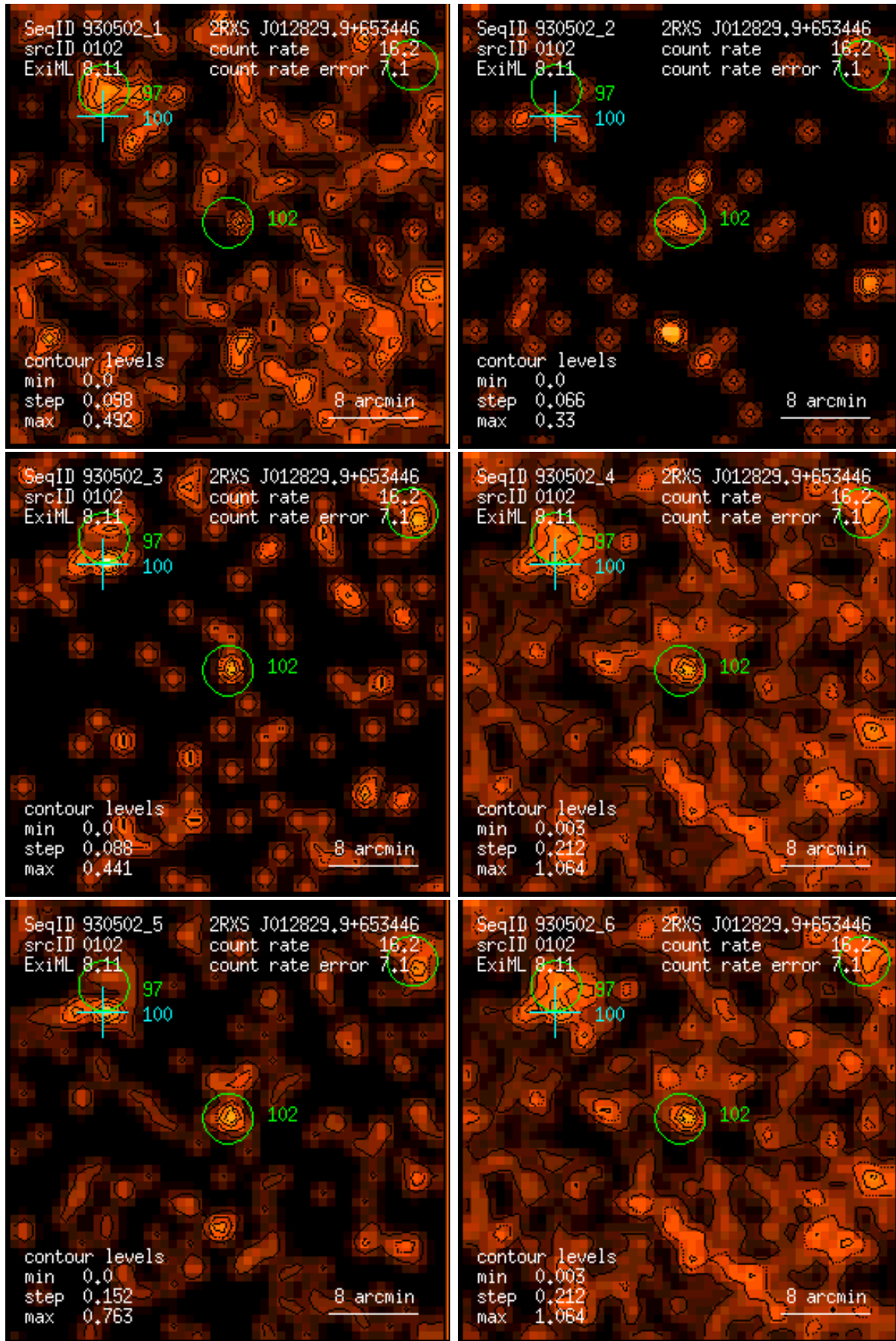
Figure 102: RASS 930502: detection 0102: band rate images, Gaussian filter: (1) PSPC channels 11 – 41, (2) 52 – 90, (3) 91 – 201, (4) 11 – 235, (5) 52 – 201, (6) 11 – 201. Broad band rates in counts/ks. Band rate contour levels in counts/ks/arcmin 2 .
