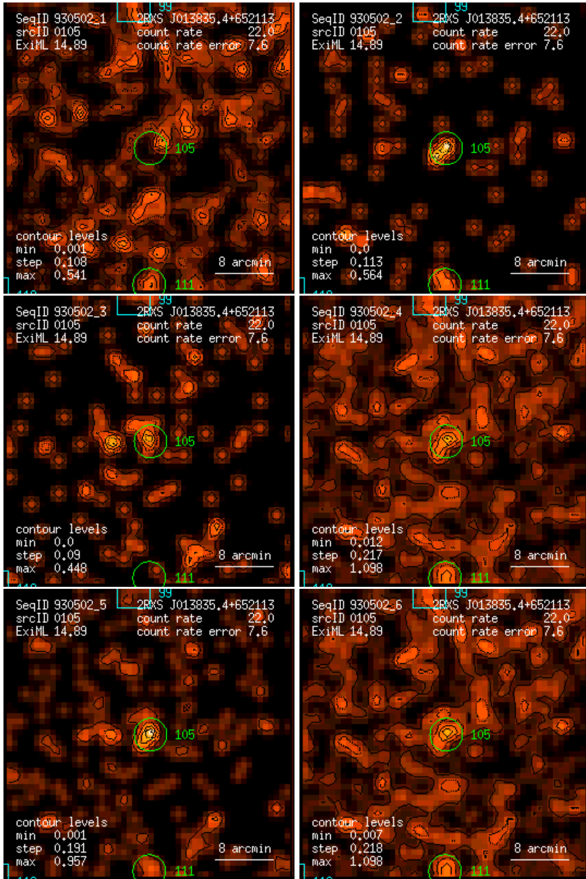
Figure 105: RASS 930502: detection 0105: band rate images, Gaussian filter: (1) PSPC channels 11 – 41, (2) 52 – 90, (3) 91 – 201, (4) 11 – 235, (5) 52 – 201, (6) 11 – 201. Broad band rates in counts/ks. Band rate contour levels in counts/ks/arcmin 2 .
