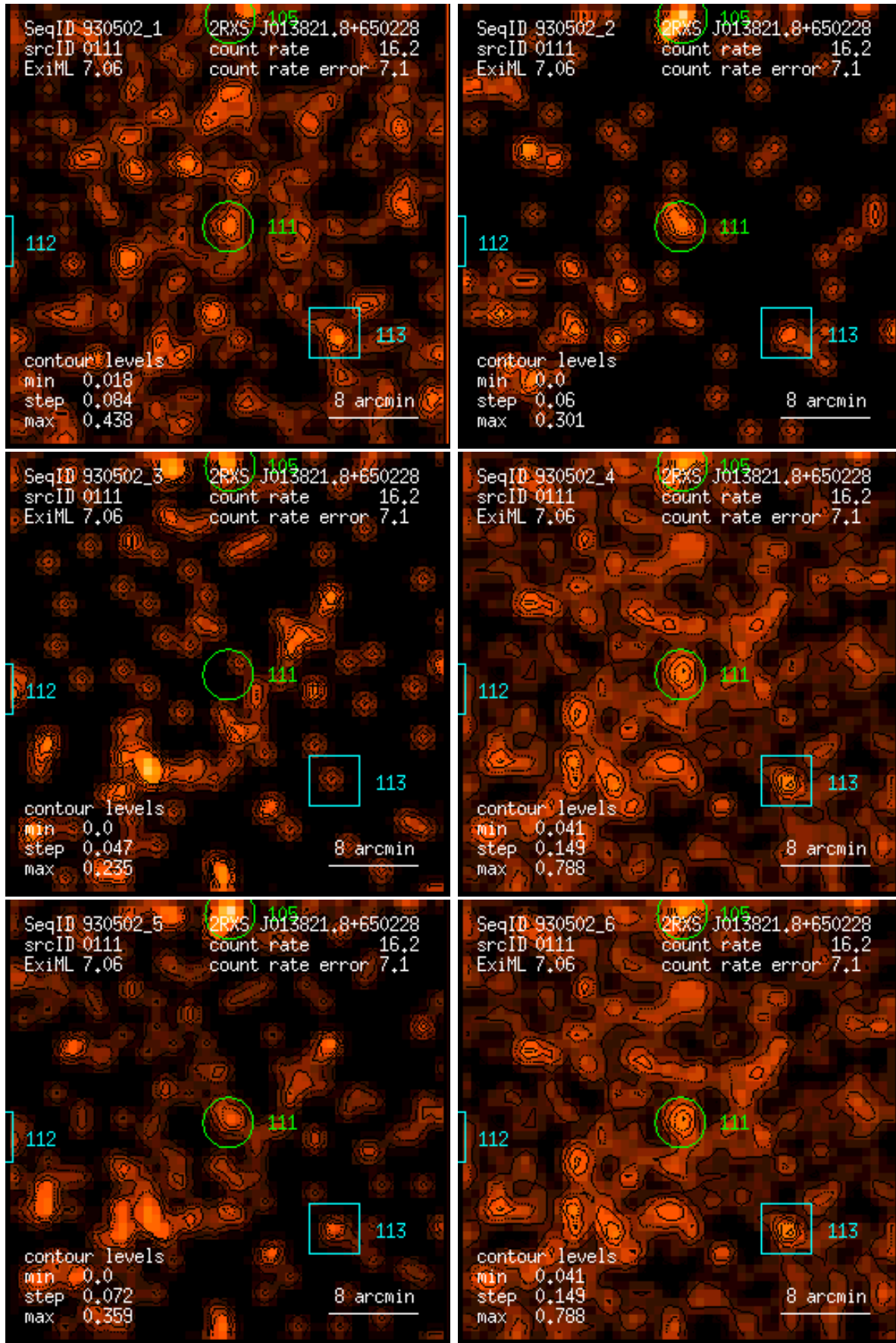
Figure 111: RASS 930502: detection 0111: band rate images, Gaussian filter: (1) PSPC channels 11 – 41, (2) 52 – 90, (3) 91 – 201, (4) 11 – 235, (5) 52 – 201, (6) 11 – 201. Broad band rates in counts/ks. Band rate contour levels in counts/ks/arcmin 2 .
