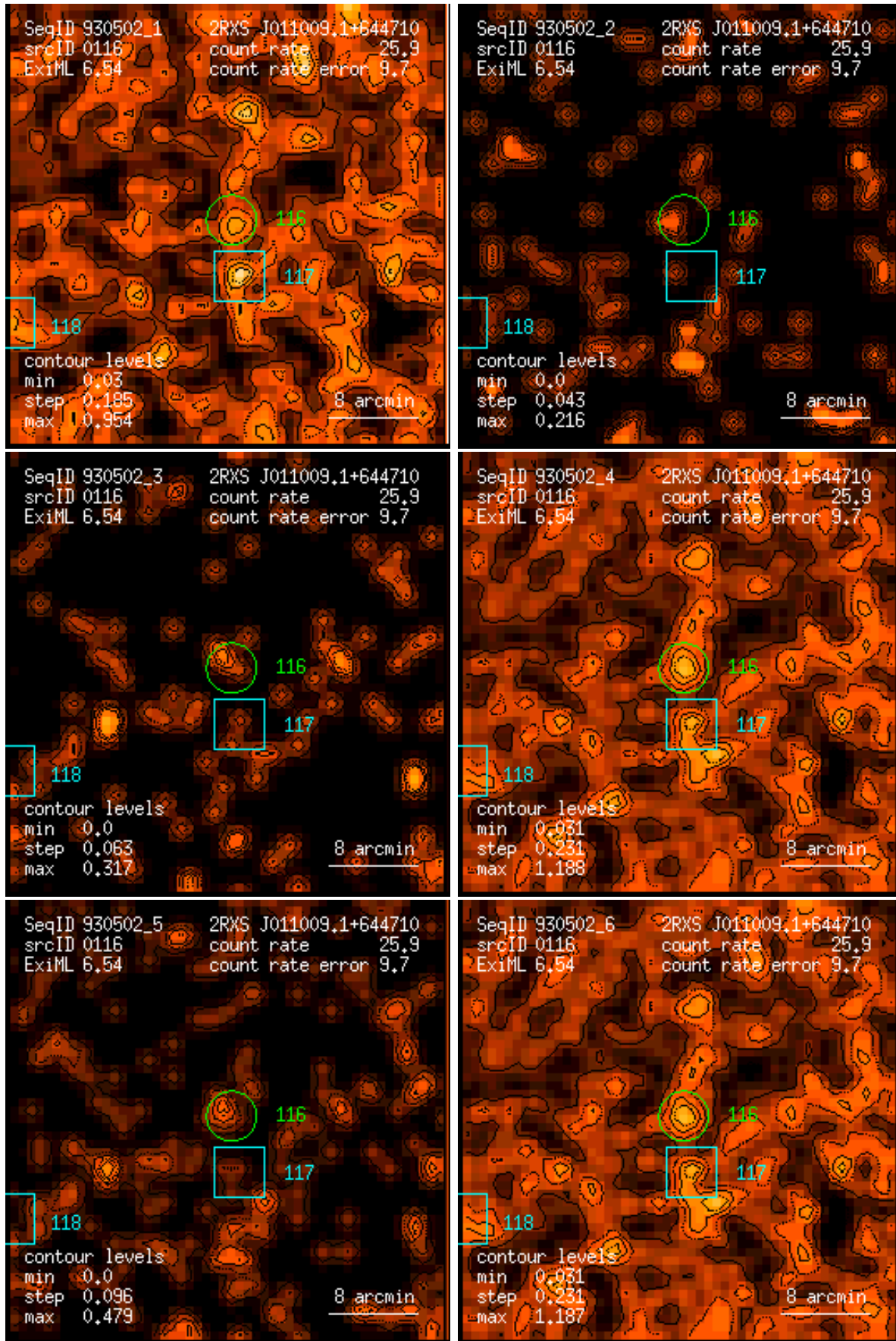
Figure 116: RASS 930502: detection 0116: band rate images, Gaussian filter: (1) PSPC channels 11 – 41, (2) 52 – 90, (3) 91 – 201, (4) 11 – 235, (5) 52 – 201, (6) 11 – 201. Broad band rates in counts/ks. Band rate contour levels in counts/ks/arcmin 2 .
