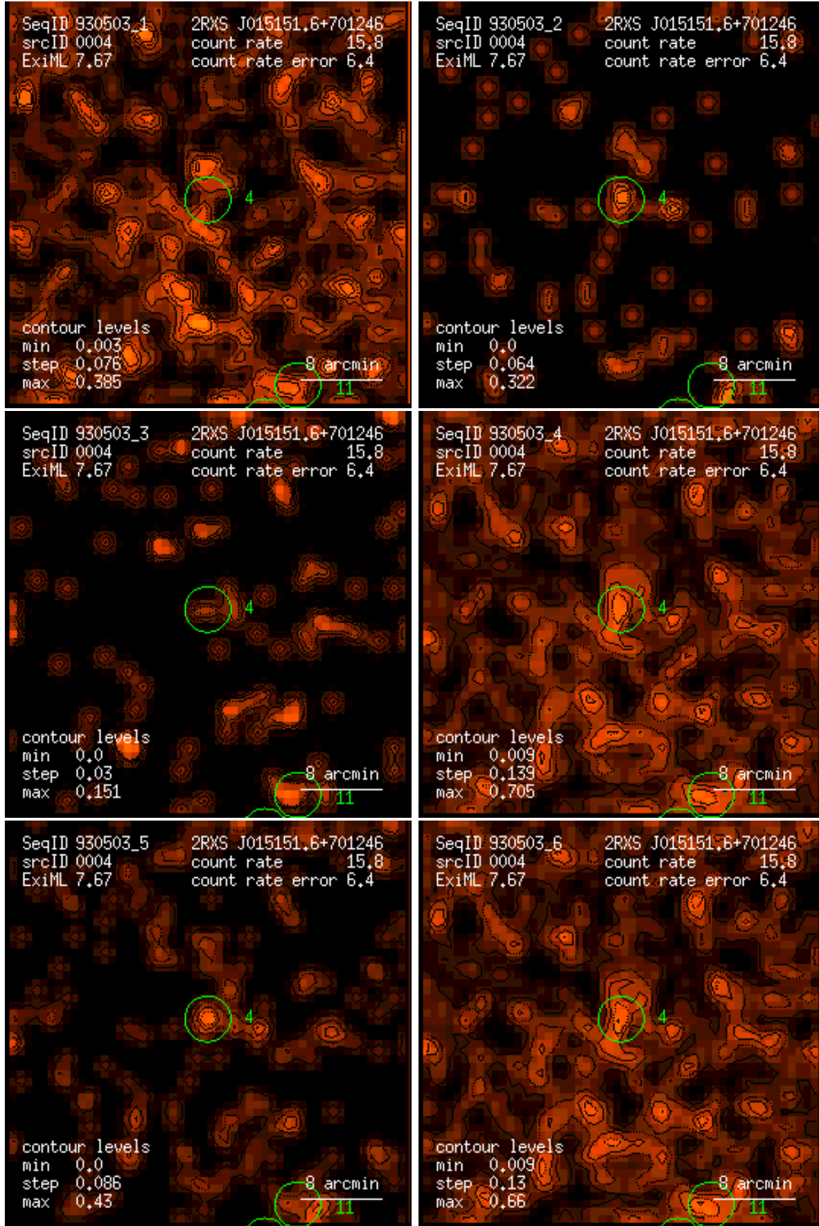
Figure 4: RASS 930503: detection 0004: band rate images, Gaussian filter: (1) PSPC channels 11 – 41, (2) 52 – 90, (3) 91 – 201, (4) 11 – 235, (5) 52 – 201, (6) 11 – 201. Broad band rates in counts/ks. Band rate contour levels in counts/ks/arcmin 2 .
