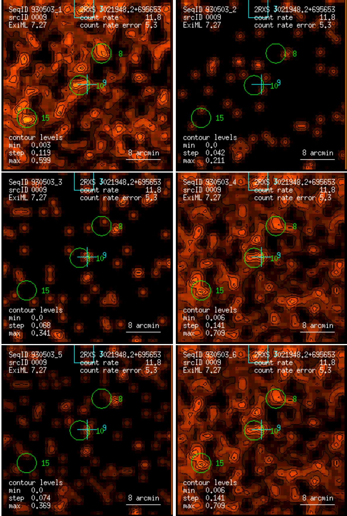
Figure 9: RASS 930503: detection 0009: band rate images, Gaussian filter: (1) PSPC channels 11 – 41, (2) 52 – 90, (3) 91 – 201, (4) 11 – 235, (5) 52 – 201, (6) 11 – 201. Broad band rates in counts/ks. Band rate contour levels in counts/ks/arcmin 2 .
