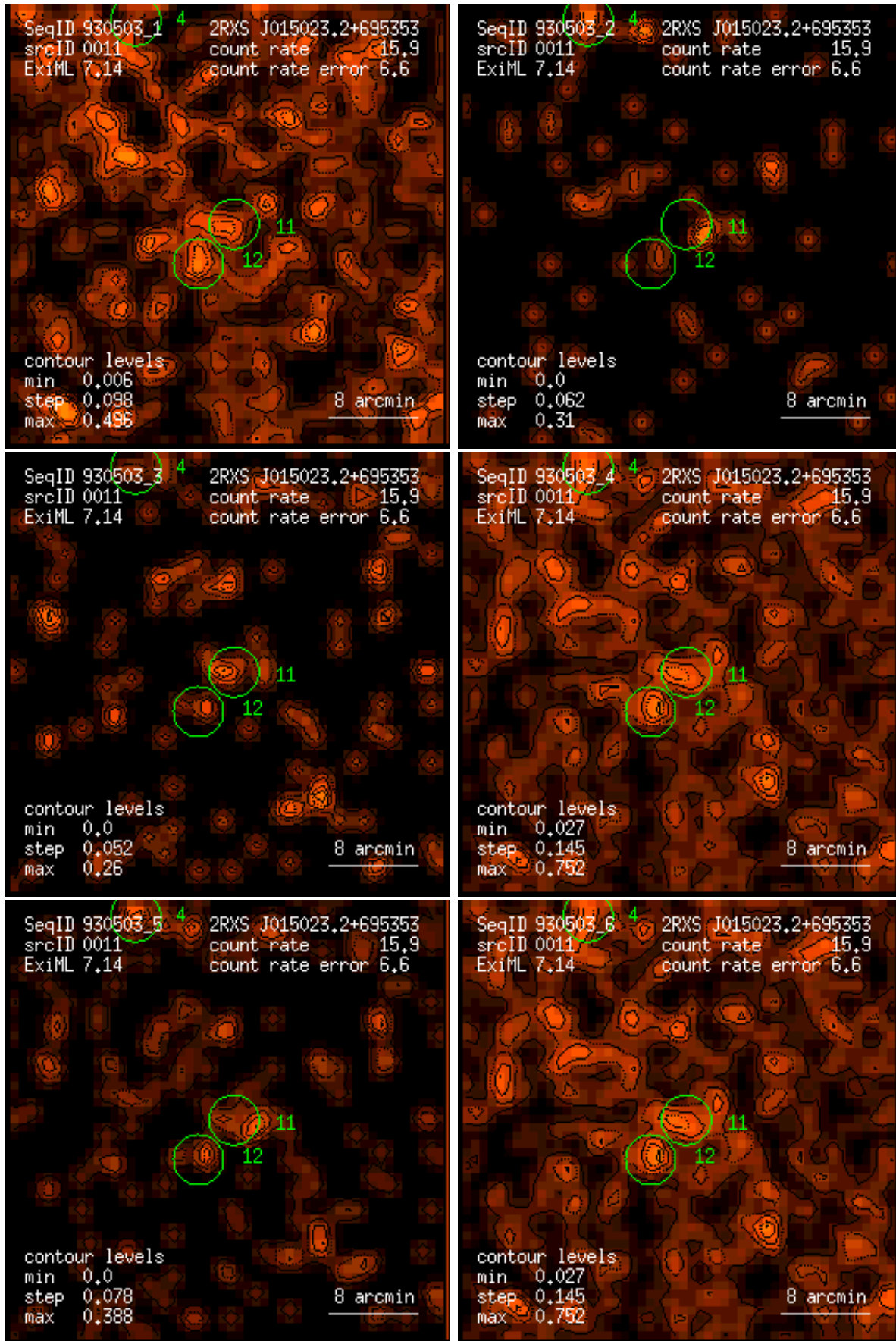
Figure 11: RASS 930503: detection 0011: band rate images, Gaussian filter: (1) PSPC channels 11 – 41, (2) 52 – 90, (3) 91 – 201, (4) 11 – 235, (5) 52 – 201, (6) 11 – 201. Broad band rates in counts/ks. Band rate contour levels in counts/ks/arcmin 2 .
