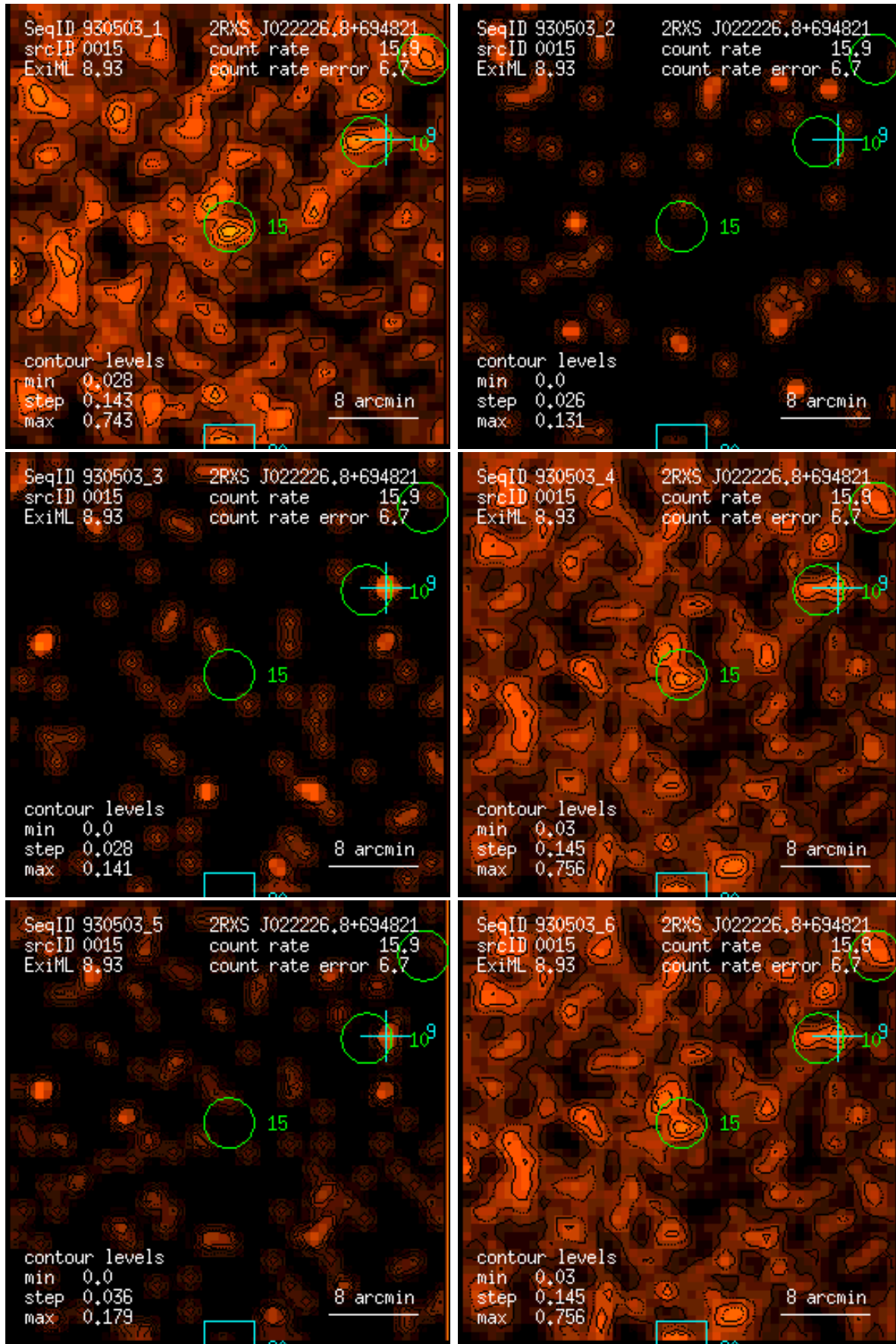
Figure 15: RASS 930503: detection 0015: band rate images, Gaussian filter: (1) PSPC channels 11 – 41, (2) 52 – 90, (3) 91 – 201, (4) 11 – 235, (5) 52 – 201, (6) 11 – 201. Broad band rates in counts/ks. Band rate contour levels in counts/ks/arcmin 2 .
