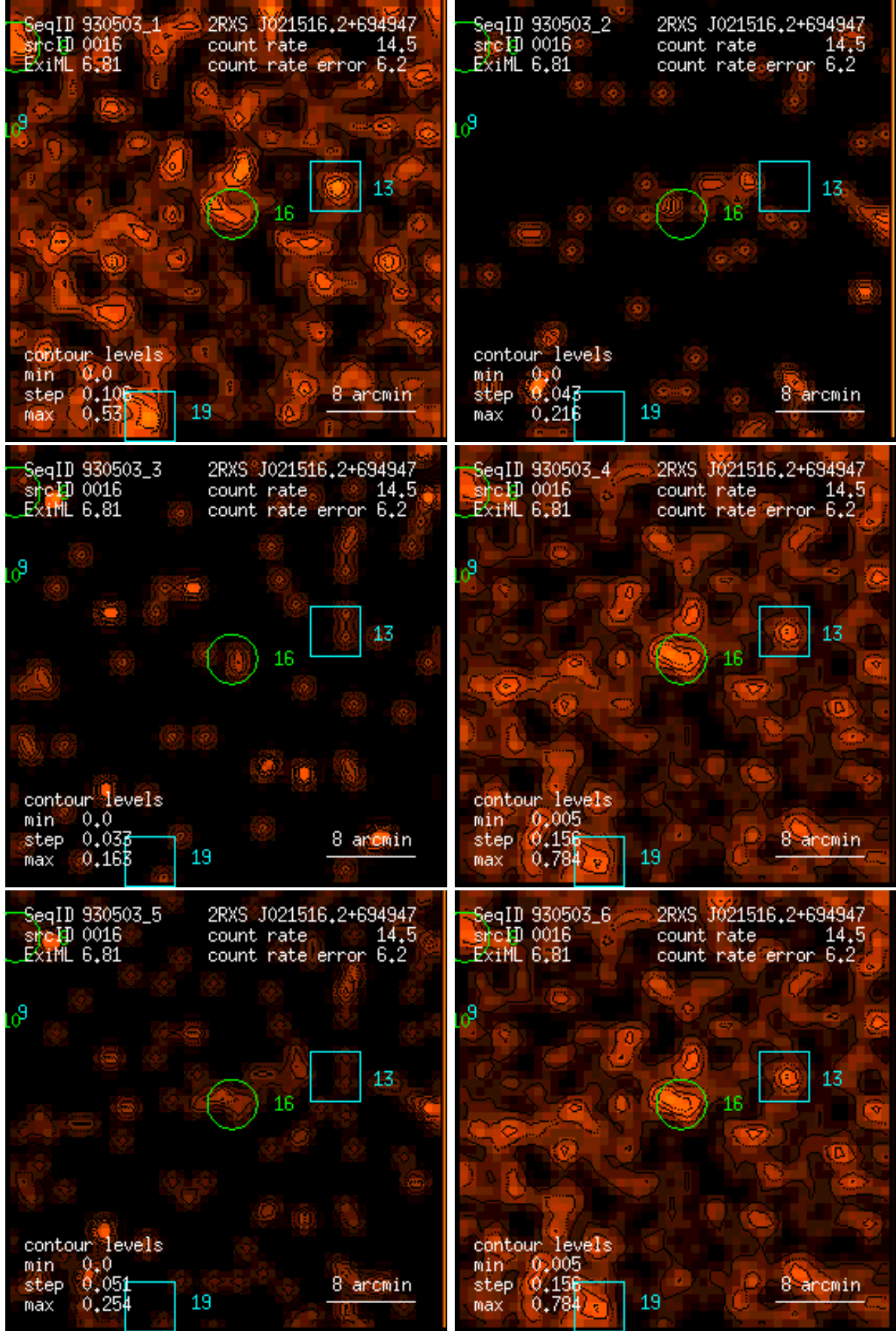
Figure 16: RASS 930503: detection 0016: band rate images, Gaussian filter: (1) PSPC channels 11 – 41, (2) 52 – 90, (3) 91 – 201, (4) 11 – 235, (5) 52 – 201, (6) 11 – 201. Broad band rates in counts/ks. Band rate contour levels in counts/ks/arcmin 2 .
