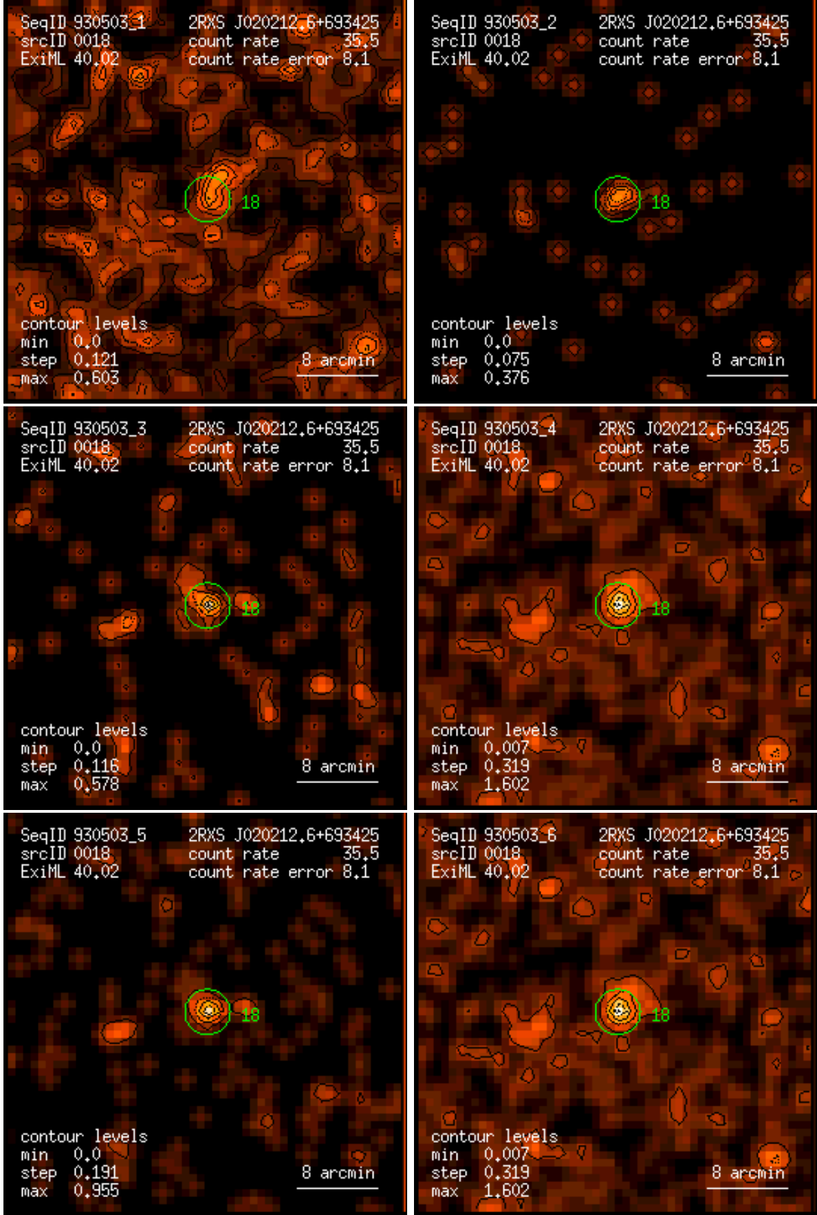
Figure 18: RASS 930503: detection 0018: band rate images, Gaussian filter: (1) PSPC channels 11 – 41, (2) 52 – 90, (3) 91 – 201, (4) 11 – 235, (5) 52 – 201, (6) 11 – 201. Broad band rates in counts/ks. Band rate contour levels in counts/ks/arcmin 2 .
