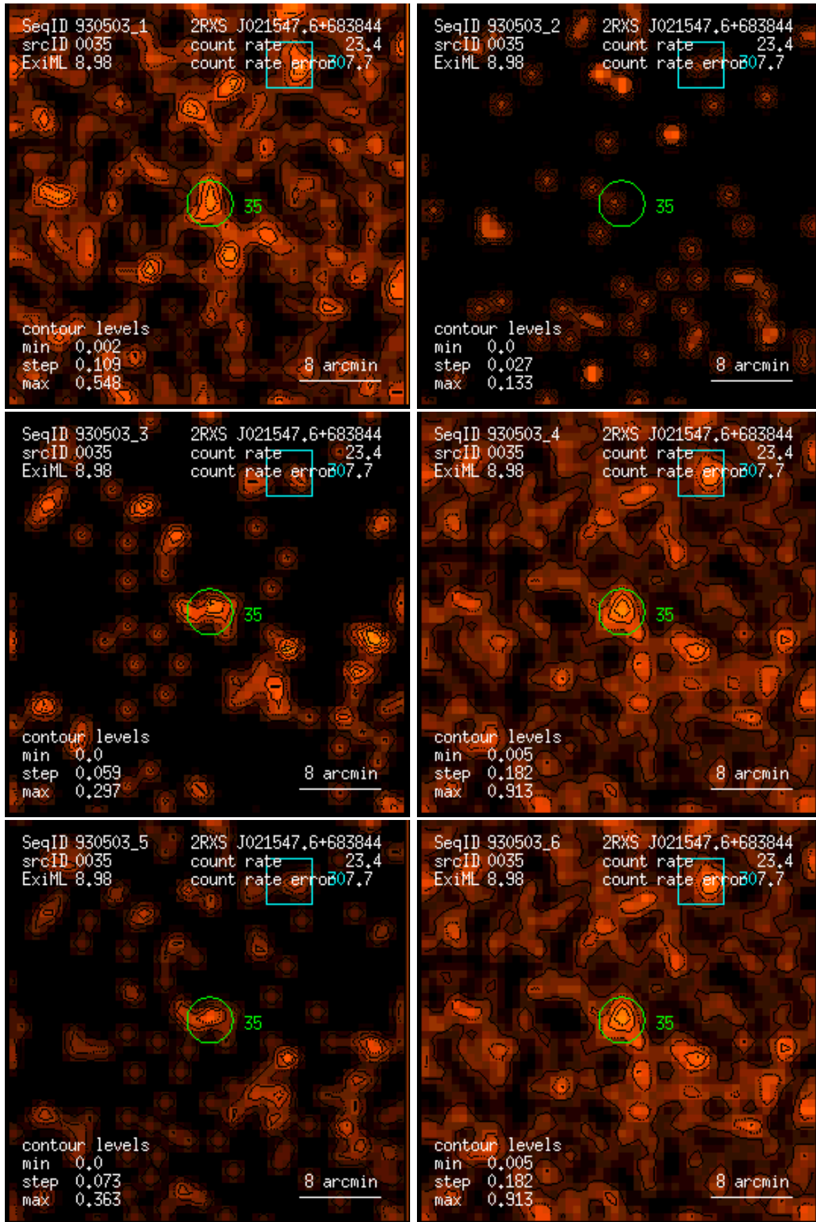
Figure 35: RASS 930503: detection 0035: band rate images, Gaussian filter: (1) PSPC channels 11 – 41, (2) 52 – 90, (3) 91 – 201, (4) 11 – 235, (5) 52 – 201, (6) 11 – 201. Broad band rates in counts/ks. Band rate contour levels in counts/ks/arcmin 2 .
