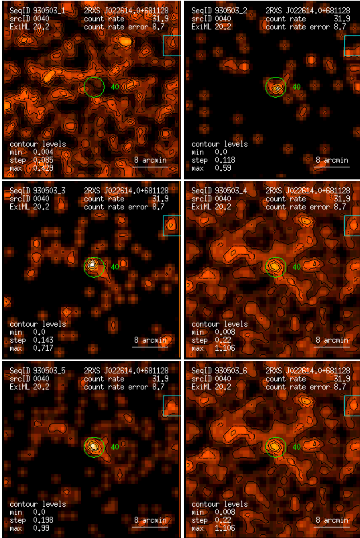
Figure 40: RASS 930503: detection 0040: band rate images, Gaussian filter: (1) PSPC channels 11 – 41, (2) 52 – 90, (3) 91 – 201, (4) 11 – 235, (5) 52 – 201, (6) 11 – 201. Broad band rates in counts/ks. Band rate contour levels in counts/ks/arcmin 2 .
