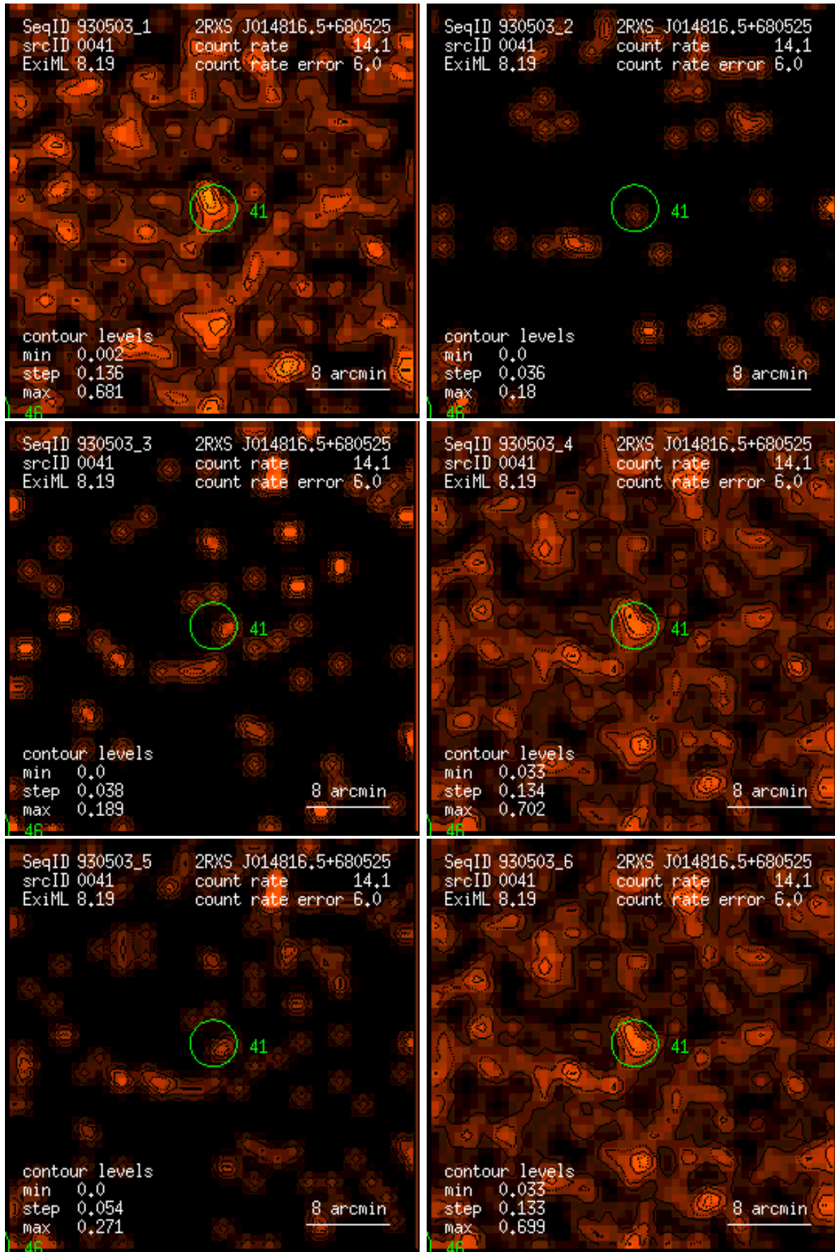
Figure 41: RASS 930503: detection 0041: band rate images, Gaussian filter: (1) PSPC channels 11 – 41, (2) 52 – 90, (3) 91 – 201, (4) 11 – 235, (5) 52 – 201, (6) 11 – 201. Broad band rates in counts/ks. Band rate contour levels in counts/ks/arcmin 2 .
