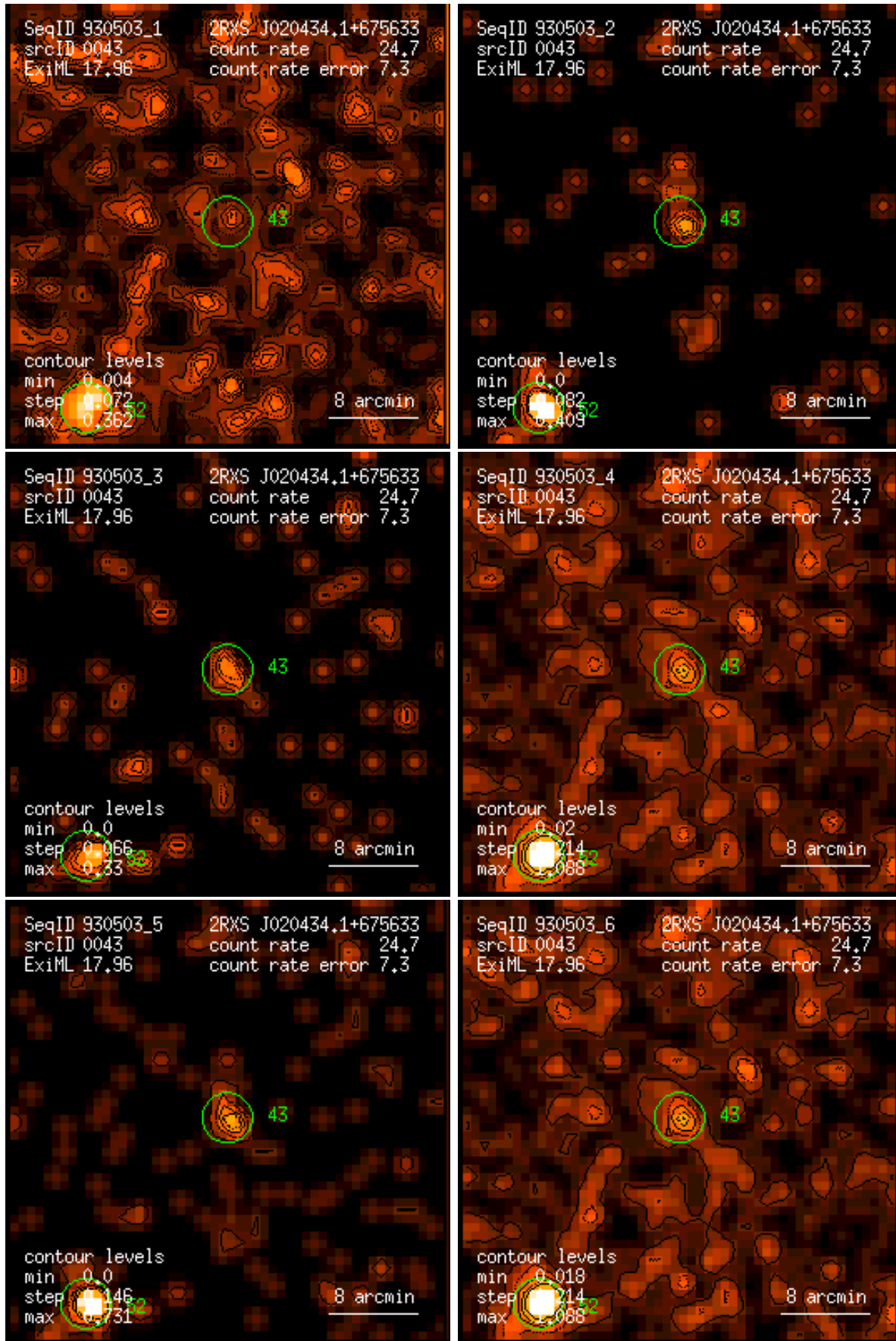
Figure 43: RASS 930503: detection 0043: band rate images, Gaussian filter: (1) PSPC channels 11 – 41, (2) 52 – 90, (3) 91 – 201, (4) 11 – 235, (5) 52 – 201, (6) 11 – 201. Broad band rates in counts/ks. Band rate contour levels in counts/ks/arcmin 2 .
