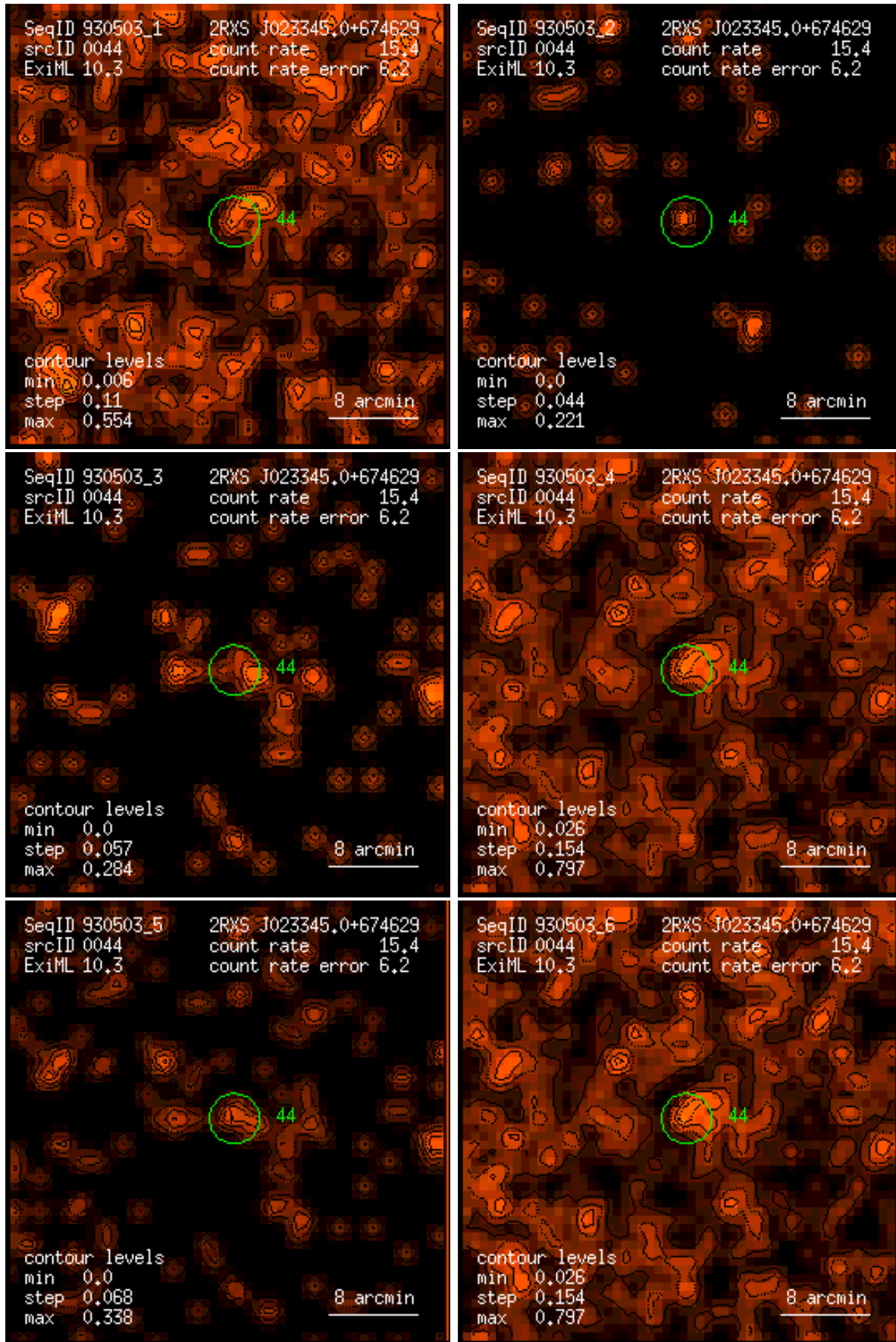
Figure 44: RASS 930503: detection 0044: band rate images, Gaussian filter: (1) PSPC channels 11 – 41, (2) 52 – 90, (3) 91 – 201, (4) 11 – 235, (5) 52 – 201, (6) 11 – 201. Broad band rates in counts/ks. Band rate contour levels in counts/ks/arcmin 2 .
