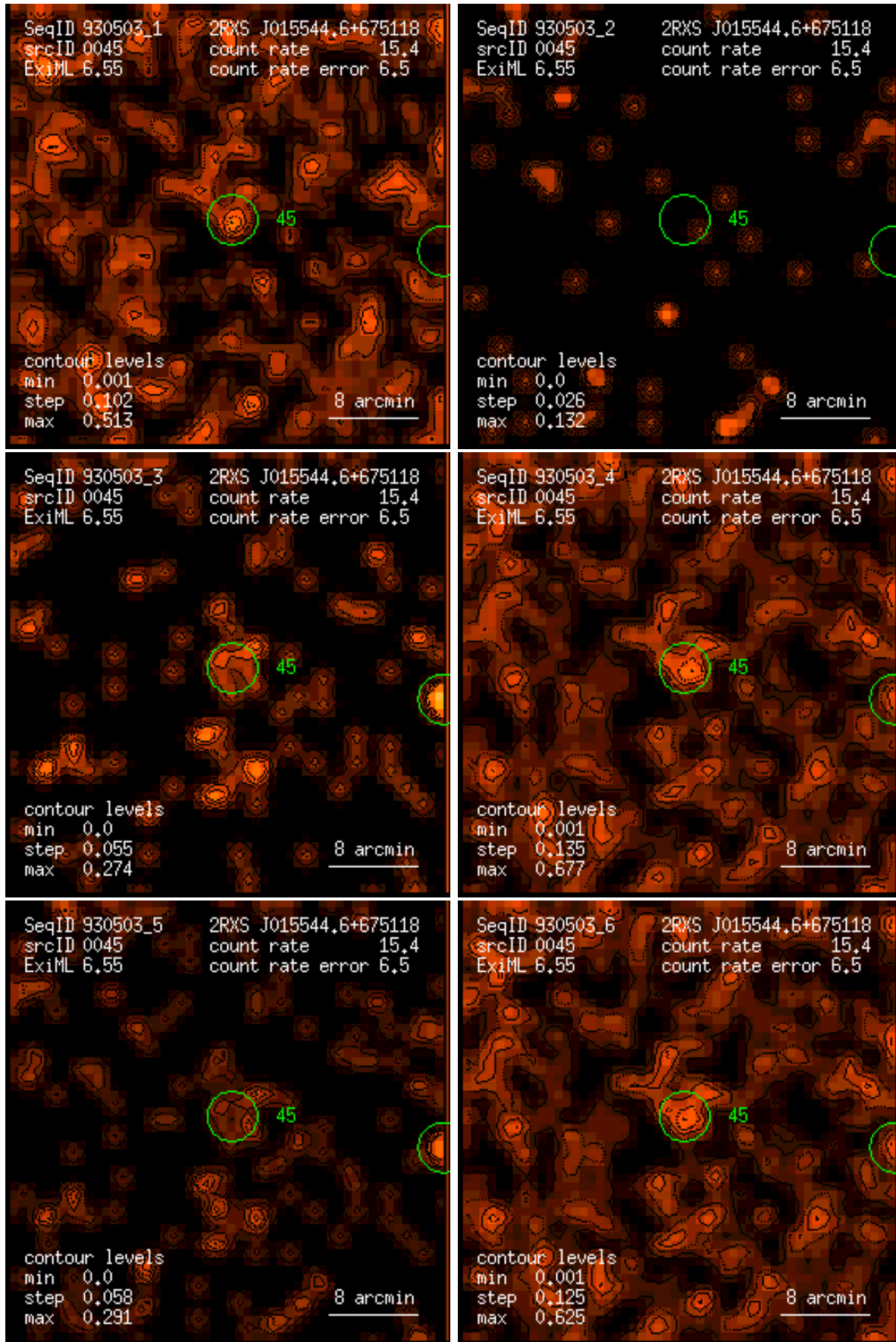
Figure 45: RASS 930503: detection 0045: band rate images, Gaussian filter: (1) PSPC channels 11 – 41, (2) 52 – 90, (3) 91 – 201, (4) 11 – 235, (5) 52 – 201, (6) 11 – 201. Broad band rates in counts/ks. Band rate contour levels in counts/ks/arcmin 2 .
