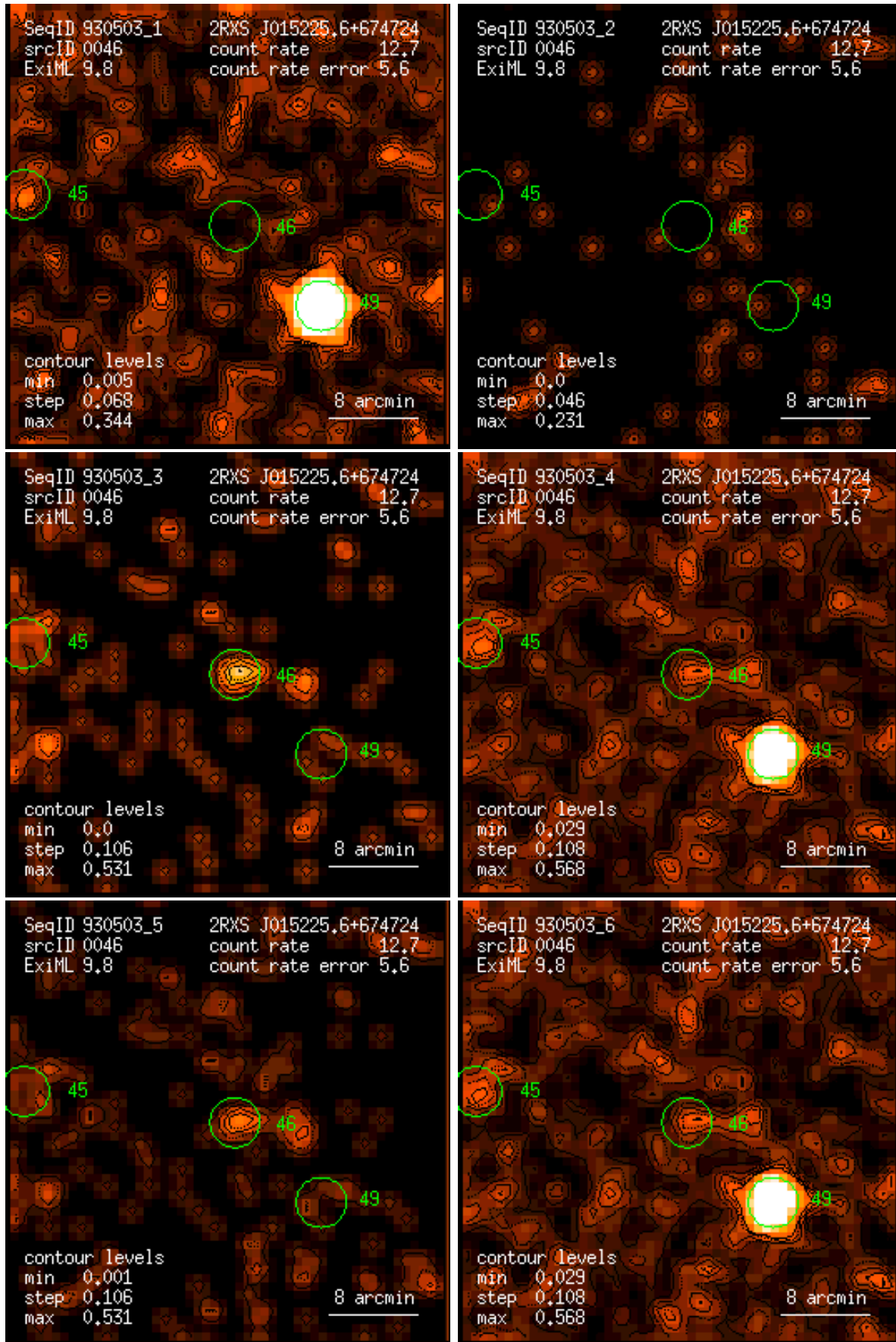
Figure 46: RASS 930503: detection 0046: band rate images, Gaussian filter: (1) PSPC channels 11 – 41, (2) 52 – 90, (3) 91 – 201, (4) 11 – 235, (5) 52 – 201, (6) 11 – 201. Broad band rates in counts/ks. Band rate contour levels in counts/ks/arcmin 2 .
