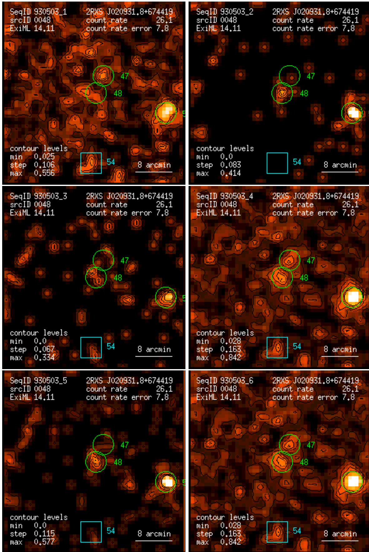
Figure 48: RASS 930503: detection 0048: band rate images, Gaussian filter: (1) PSPC channels 11 – 41, (2) 52 – 90, (3) 91 – 201, (4) 11 – 235, (5) 52 – 201, (6) 11 – 201. Broad band rates in counts/ks. Band rate contour levels in counts/ks/arcmin 2 .
