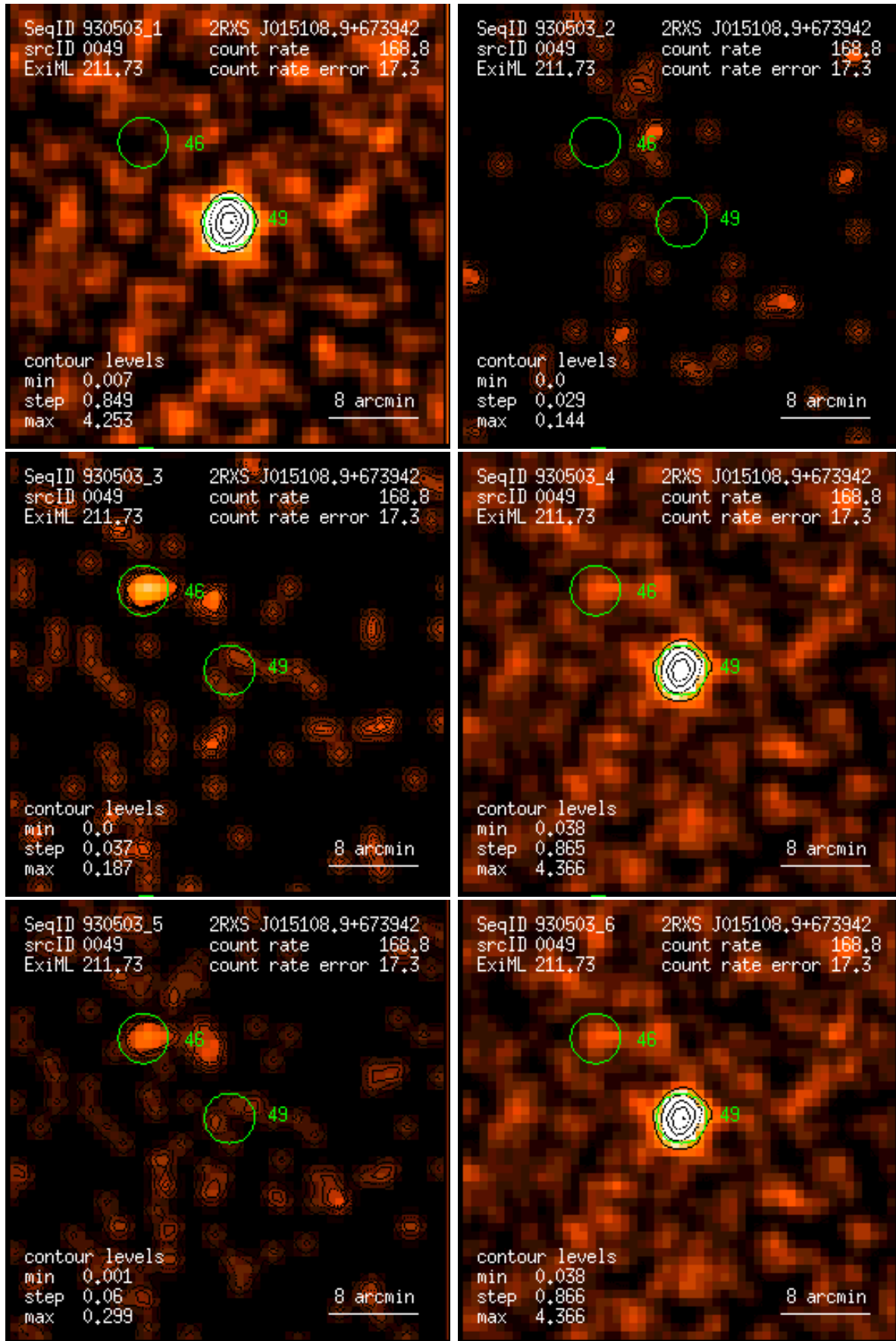
Figure 49: RASS 930503: detection 0049: band rate images, Gaussian filter: (1) PSPC channels 11 – 41, (2) 52 – 90, (3) 91 – 201, (4) 11 – 235, (5) 52 – 201, (6) 11 – 201. Broad band rates in counts/ks. Band rate contour levels in counts/ks/arcmin 2 .
