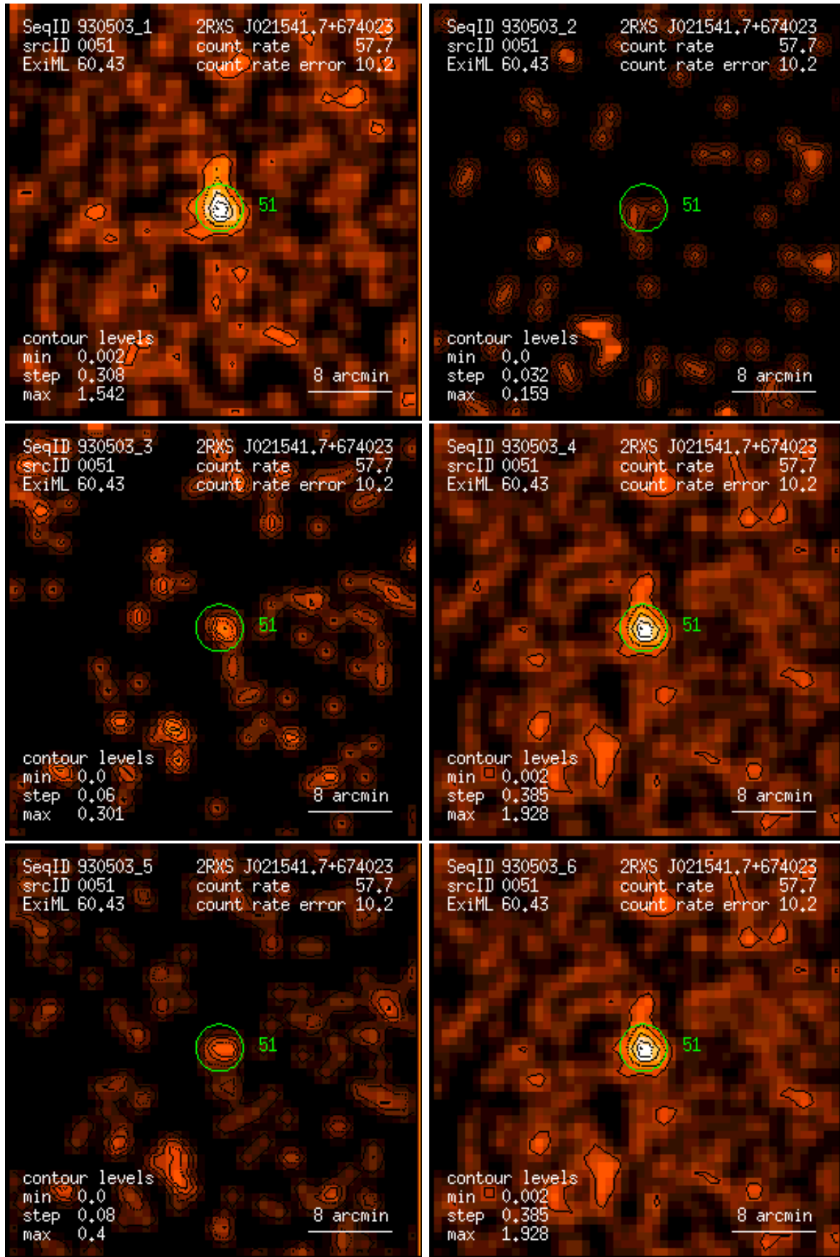
Figure 51: RASS 930503: detection 0051: band rate images, Gaussian filter: (1) PSPC channels 11 – 41, (2) 52 – 90, (3) 91 – 201, (4) 11 – 235, (5) 52 – 201, (6) 11 – 201. Broad band rates in counts/ks. Band rate contour levels in counts/ks/arcmin 2 .
