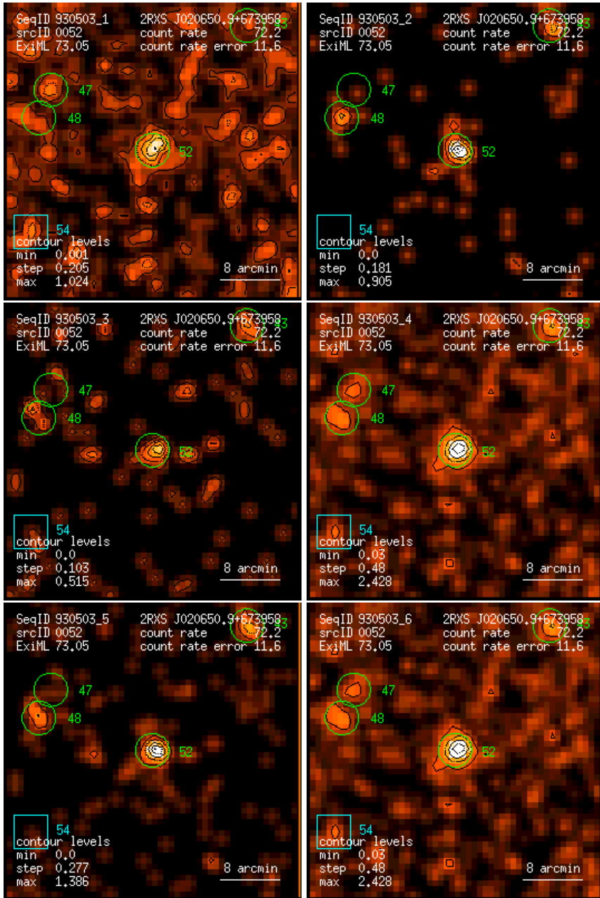
Figure 52: RASS 930503: detection 0052: band rate images, Gaussian filter: (1) PSPC channels 11 – 41, (2) 52 – 90, (3) 91 – 201, (4) 11 – 235, (5) 52 – 201, (6) 11 – 201. Broad band rates in counts/ks. Band rate contour levels in counts/ks/arcmin 2 .
