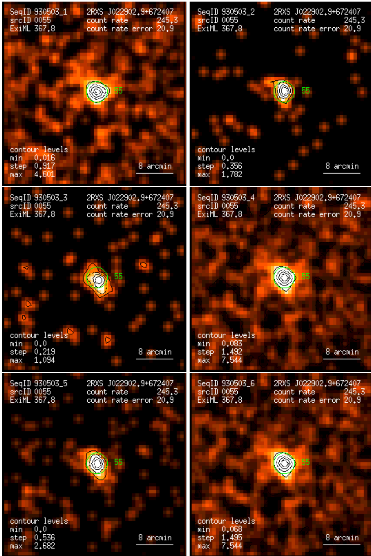
Figure 55: RASS 930503: detection 0055: band rate images, Gaussian filter: (1) PSPC channels 11 – 41, (2) 52 – 90, (3) 91 – 201, (4) 11 – 235, (5) 52 – 201, (6) 11 – 201. Broad band rates in counts/ks. Band rate contour levels in counts/ks/arcmin 2 .
