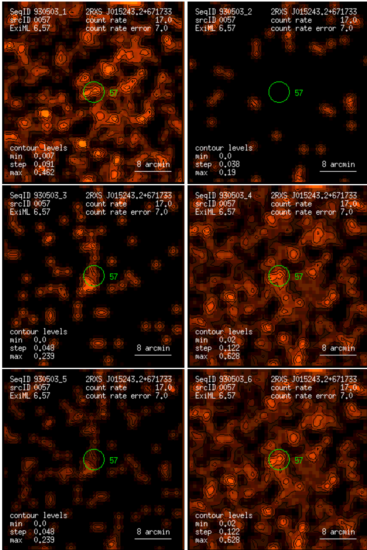
Figure 57: RASS 930503: detection 0057: band rate images, Gaussian filter: (1) PSPC channels 11 – 41, (2) 52 – 90, (3) 91 – 201, (4) 11 – 235, (5) 52 – 201, (6) 11 – 201. Broad band rates in counts/ks. Band rate contour levels in counts/ks/arcmin 2 .
