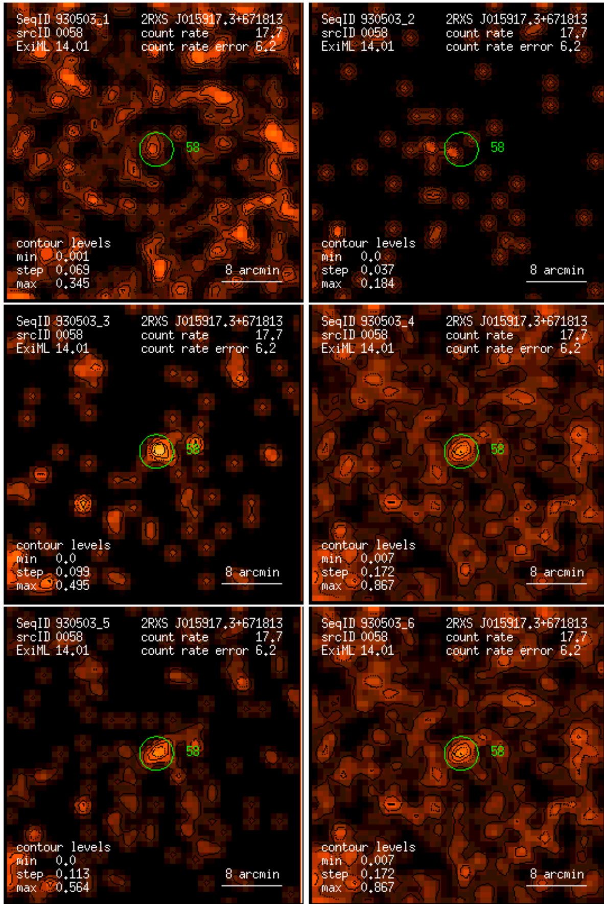
Figure 58: RASS 930503: detection 0058: band rate images, Gaussian filter: (1) PSPC channels 11 – 41, (2) 52 – 90, (3) 91 – 201, (4) 11 – 235, (5) 52 – 201, (6) 11 – 201. Broad band rates in counts/ks. Band rate contour levels in counts/ks/arcmin 2 .
