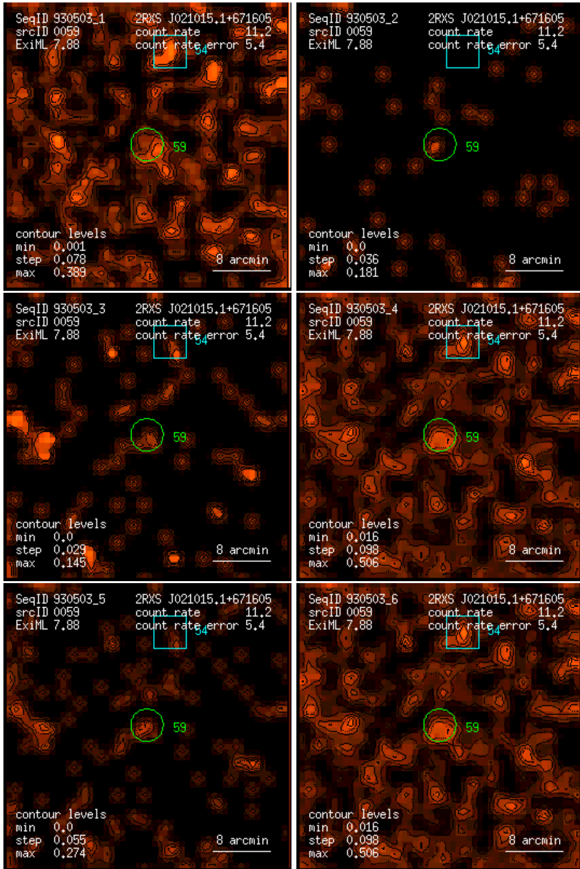
Figure 59: RASS 930503: detection 0059: band rate images, Gaussian filter: (1) PSPC channels 11 – 41, (2) 52 – 90, (3) 91 – 201, (4) 11 – 235, (5) 52 – 201, (6) 11 – 201. Broad band rates in counts/ks. Band rate contour levels in counts/ks/arcmin 2 .
