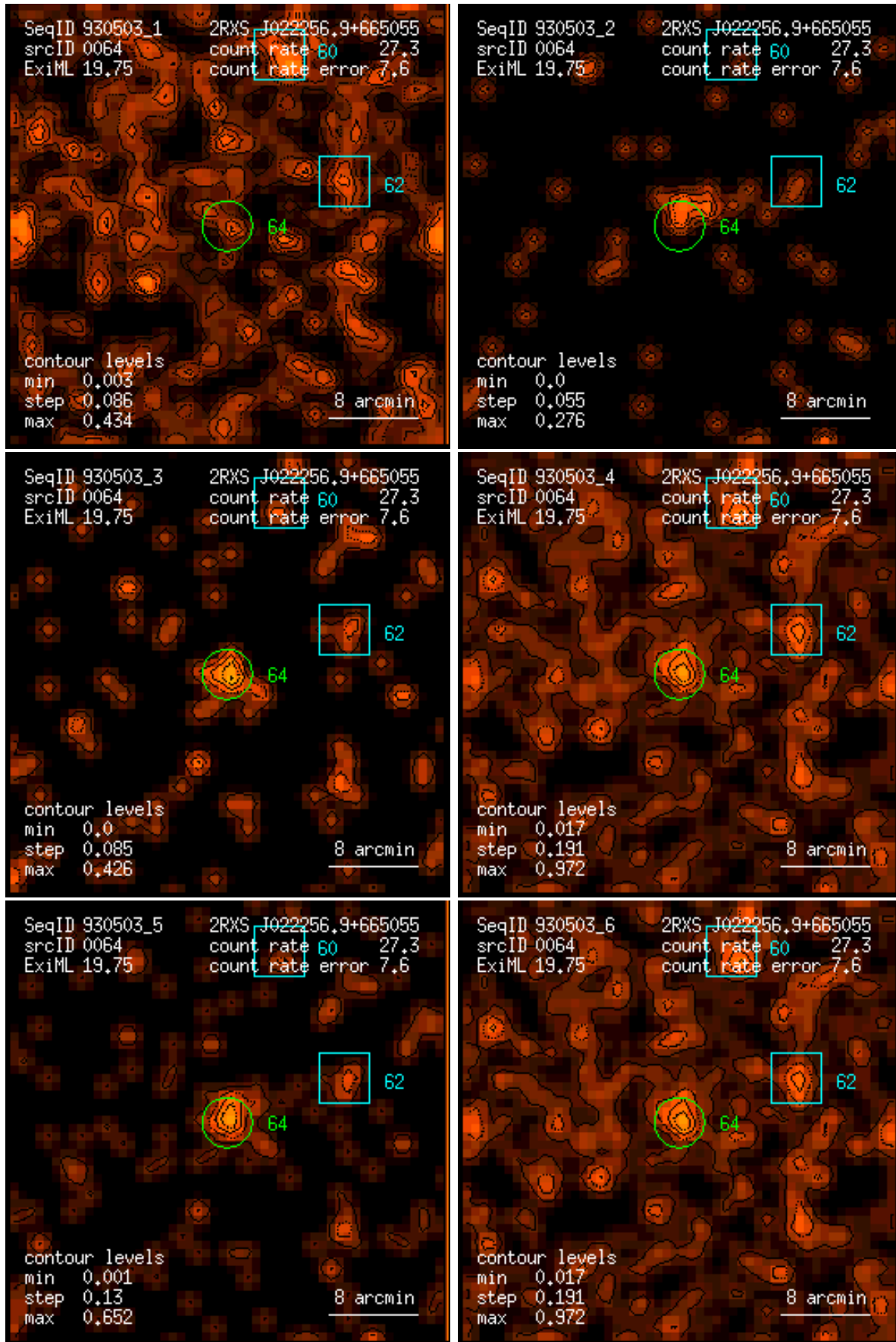
Figure 64: RASS 930503: detection 0064: band rate images, Gaussian filter: (1) PSPC channels 11 – 41, (2) 52 – 90, (3) 91 – 201, (4) 11 – 235, (5) 52 – 201, (6) 11 – 201. Broad band rates in counts/ks. Band rate contour levels in counts/ks/arcmin 2 .
