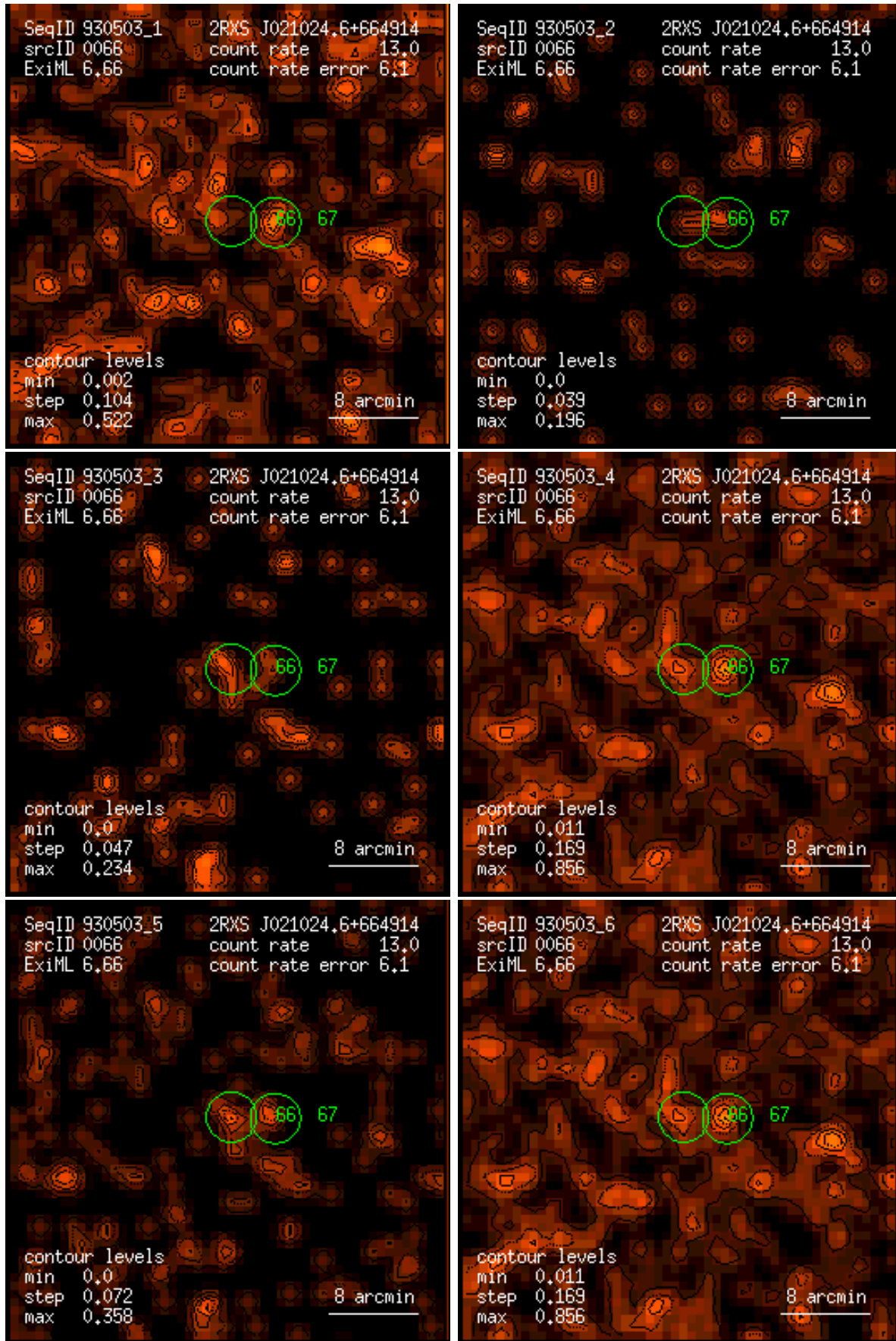
Figure 66: RASS 930503: detection 0066: band rate images, Gaussian filter: (1) PSPC channels 11 – 41, (2) 52 – 90, (3) 91 – 201, (4) 11 – 235, (5) 52 – 201, (6) 11 – 201. Broad band rates in counts/ks. Band rate contour levels in counts/ks/arcmin 2 .
