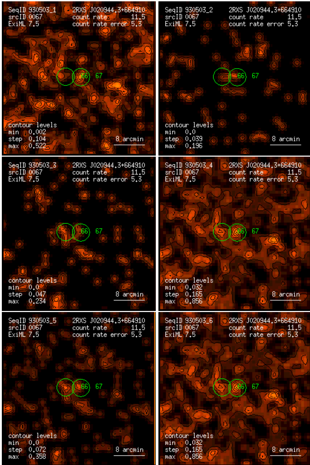
Figure 67: RASS 930503: detection 0067: band rate images, Gaussian filter: (1) PSPC channels 11 – 41, (2) 52 – 90, (3) 91 – 201, (4) 11 – 235, (5) 52 – 201, (6) 11 – 201. Broad band rates in counts/ks. Band rate contour levels in counts/ks/arcmin 2 .
