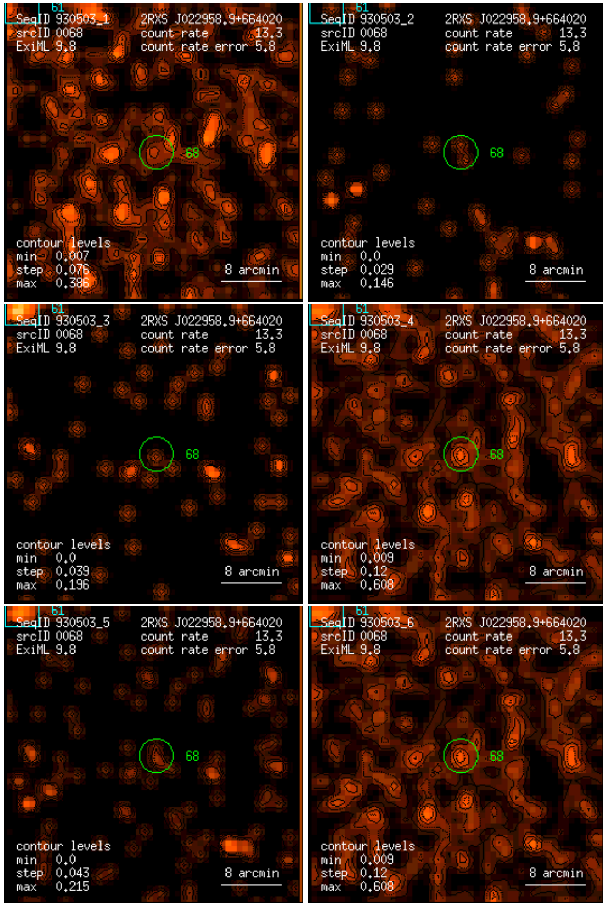
Figure 68: RASS 930503: detection 0068: band rate images, Gaussian filter: (1) PSPC channels 11 – 41, (2) 52 – 90, (3) 91 – 201, (4) 11 – 235, (5) 52 – 201, (6) 11 – 201. Broad band rates in counts/ks. Band rate contour levels in counts/ks/arcmin 2 .
