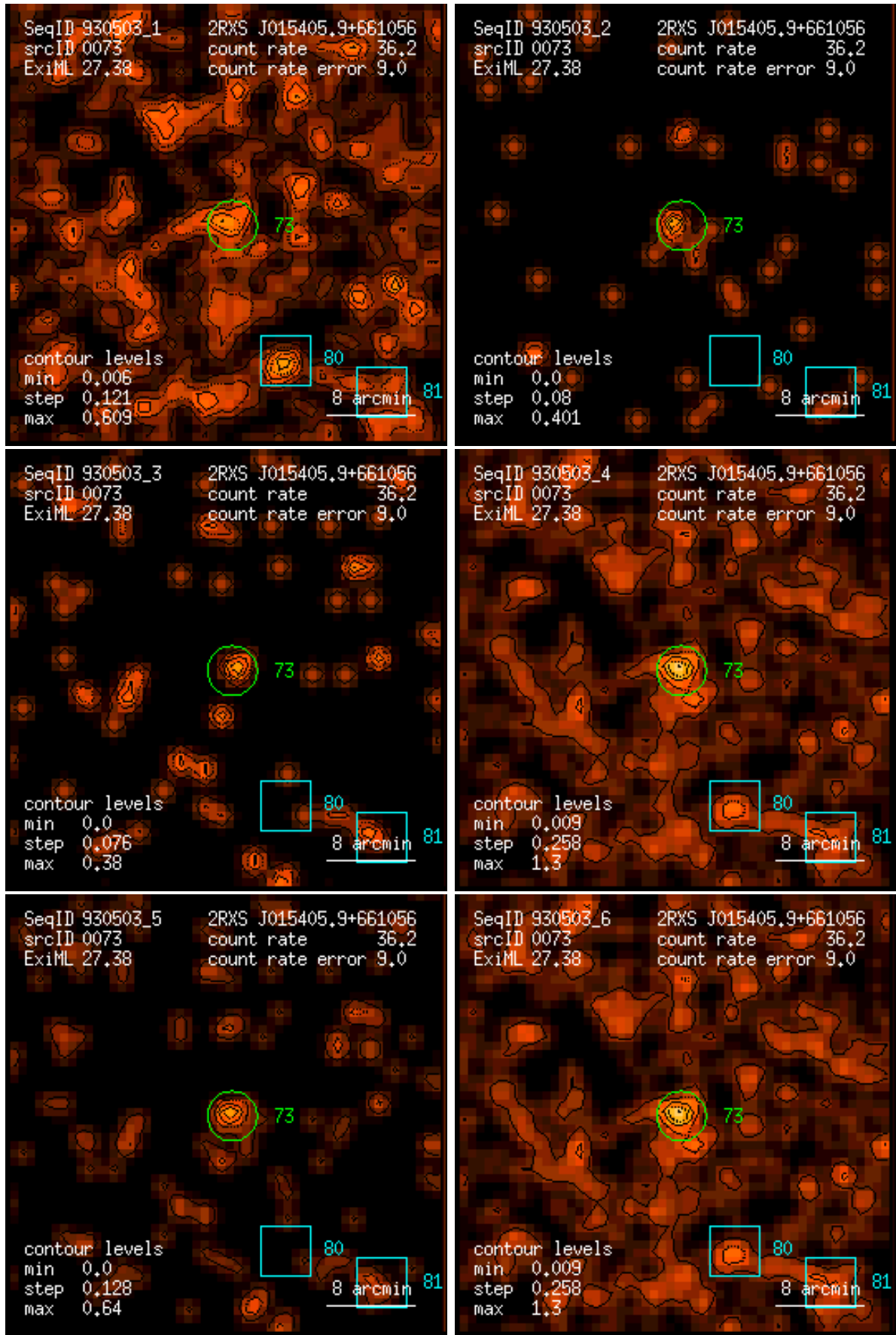
Figure 73: RASS 930503: detection 0073: band rate images, Gaussian filter: (1) PSPC channels 11 – 41, (2) 52 – 90, (3) 91 – 201, (4) 11 – 235, (5) 52 – 201, (6) 11 – 201. Broad band rates in counts/ks. Band rate contour levels in counts/ks/arcmin 2 .
