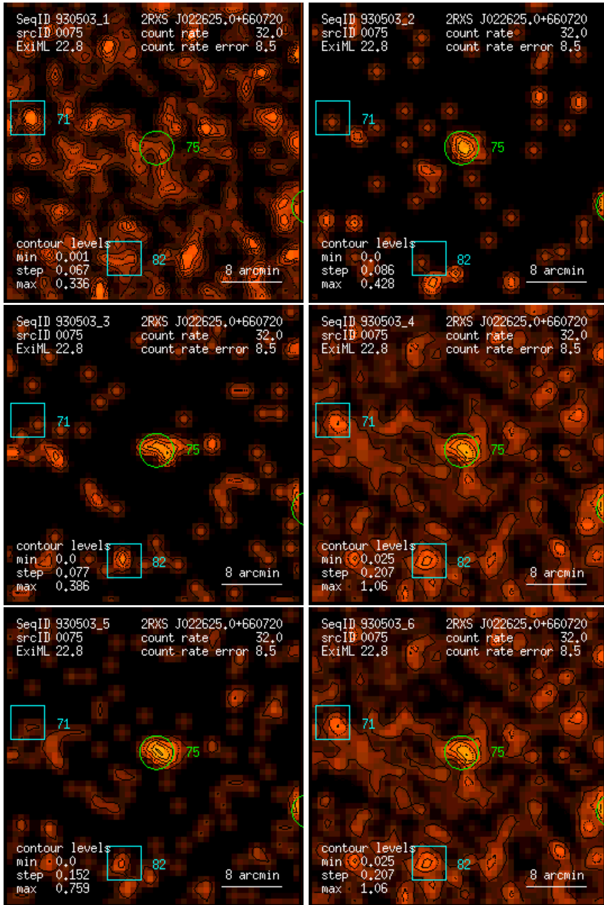
Figure 75: RASS 930503: detection 0075: band rate images, Gaussian filter: (1) PSPC channels 11 – 41, (2) 52 – 90, (3) 91 – 201, (4) 11 – 235, (5) 52 – 201, (6) 11 – 201. Broad band rates in counts/ks. Band rate contour levels in counts/ks/arcmin 2 .
