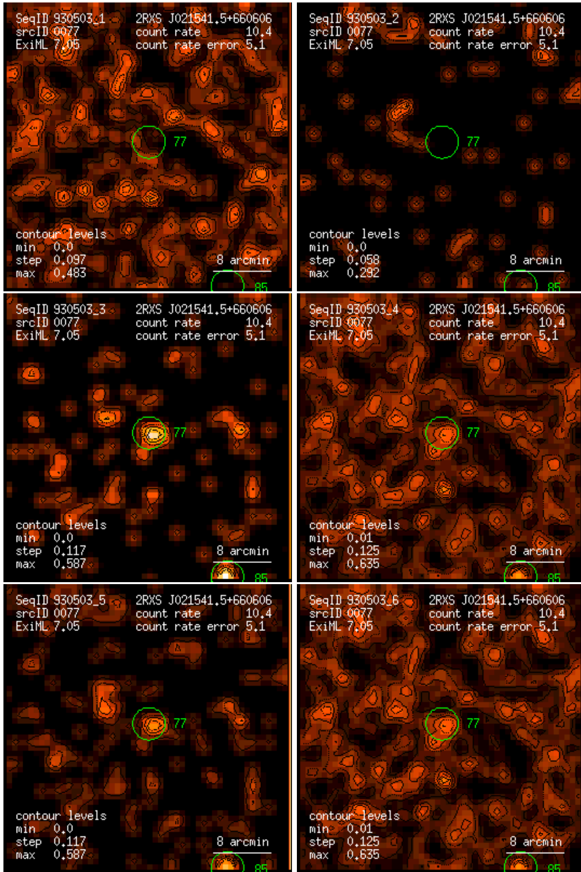
Figure 77: RASS 930503: detection 0077: band rate images, Gaussian filter: (1) PSPC channels 11 – 41, (2) 52 – 90, (3) 91 – 201, (4) 11 – 235, (5) 52 – 201, (6) 11 – 201. Broad band rates in counts/ks. Band rate contour levels in counts/ks/arcmin 2 .
