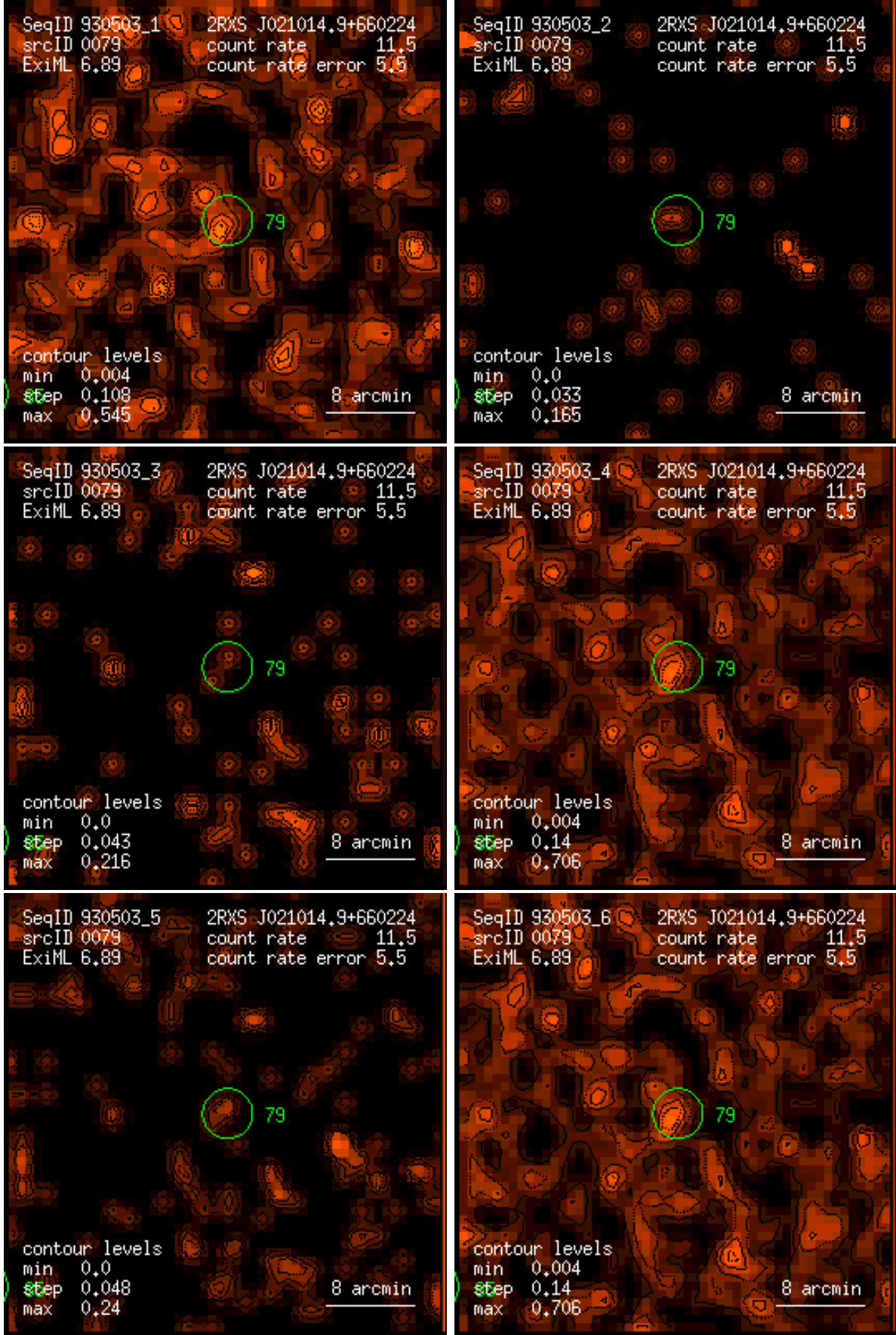
Figure 79: RASS 930503: detection 0079: band rate images, Gaussian filter: (1) PSPC channels 11 – 41, (2) 52 – 90, (3) 91 – 201, (4) 11 – 235, (5) 52 – 201, (6) 11 – 201. Broad band rates in counts/ks. Band rate contour levels in counts/ks/arcmin 2 .
